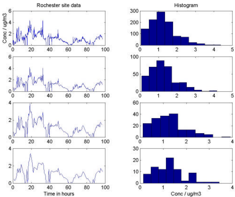
Figure 49 - Histogram (frequency - concentration) plots for formaldehyde at Rochester (averaging periods of 5, 15, 30 and 60 minutes are given top - bottom)
