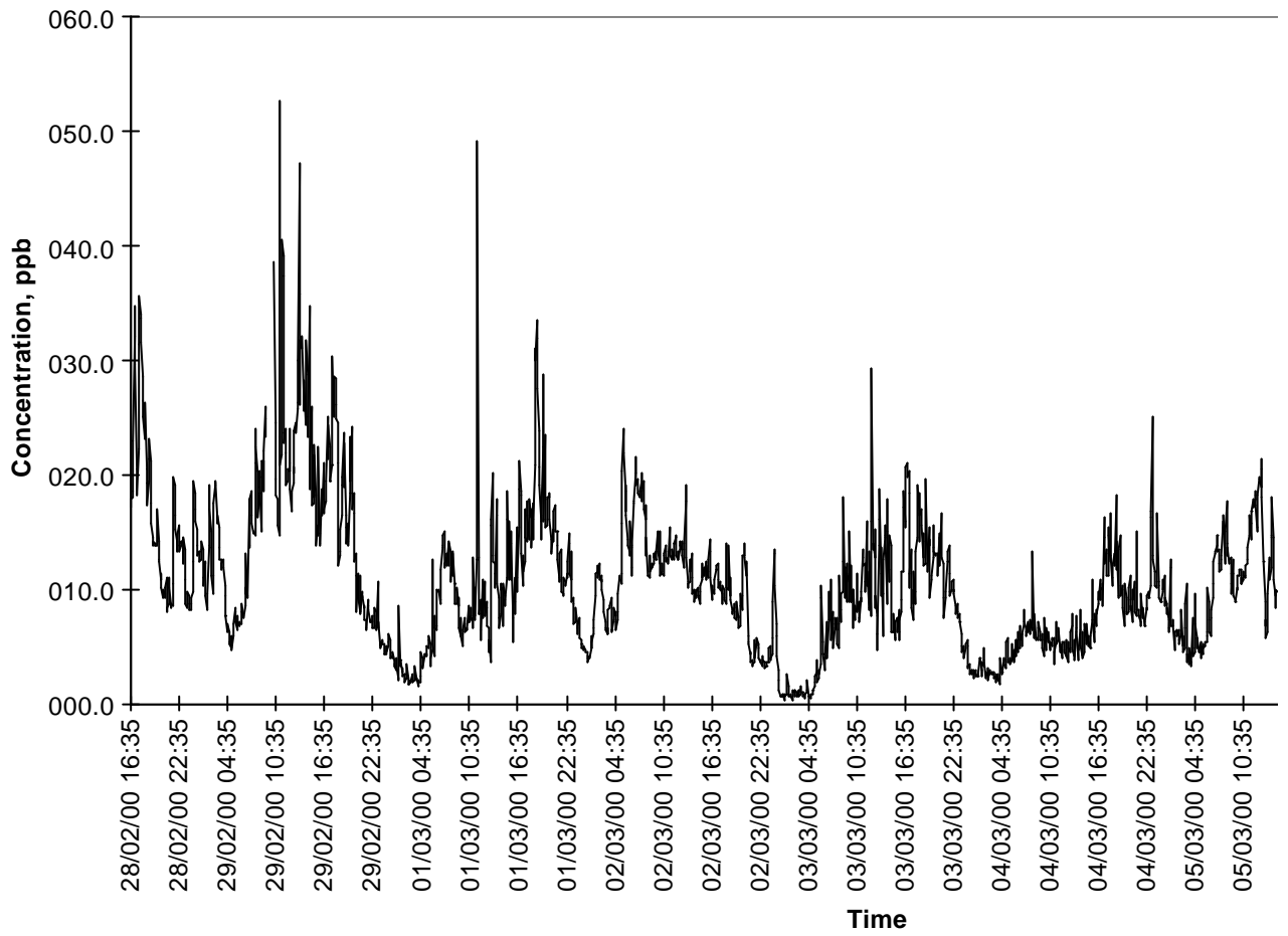
Figure 53 Time series of NO 2 measurements at an industrial site.
