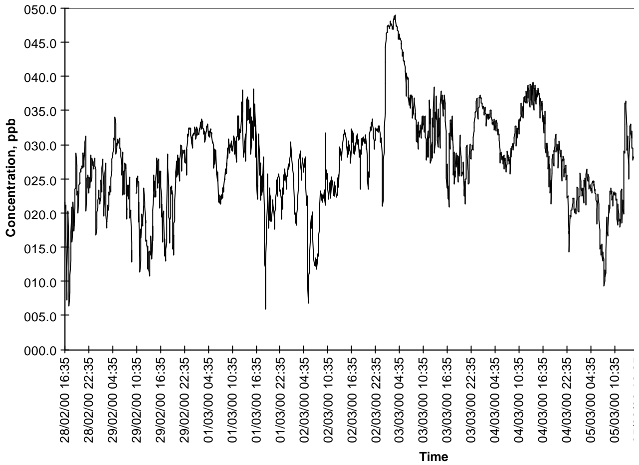
Figure 54 Time series of O 3 measurements at an industrial site.
