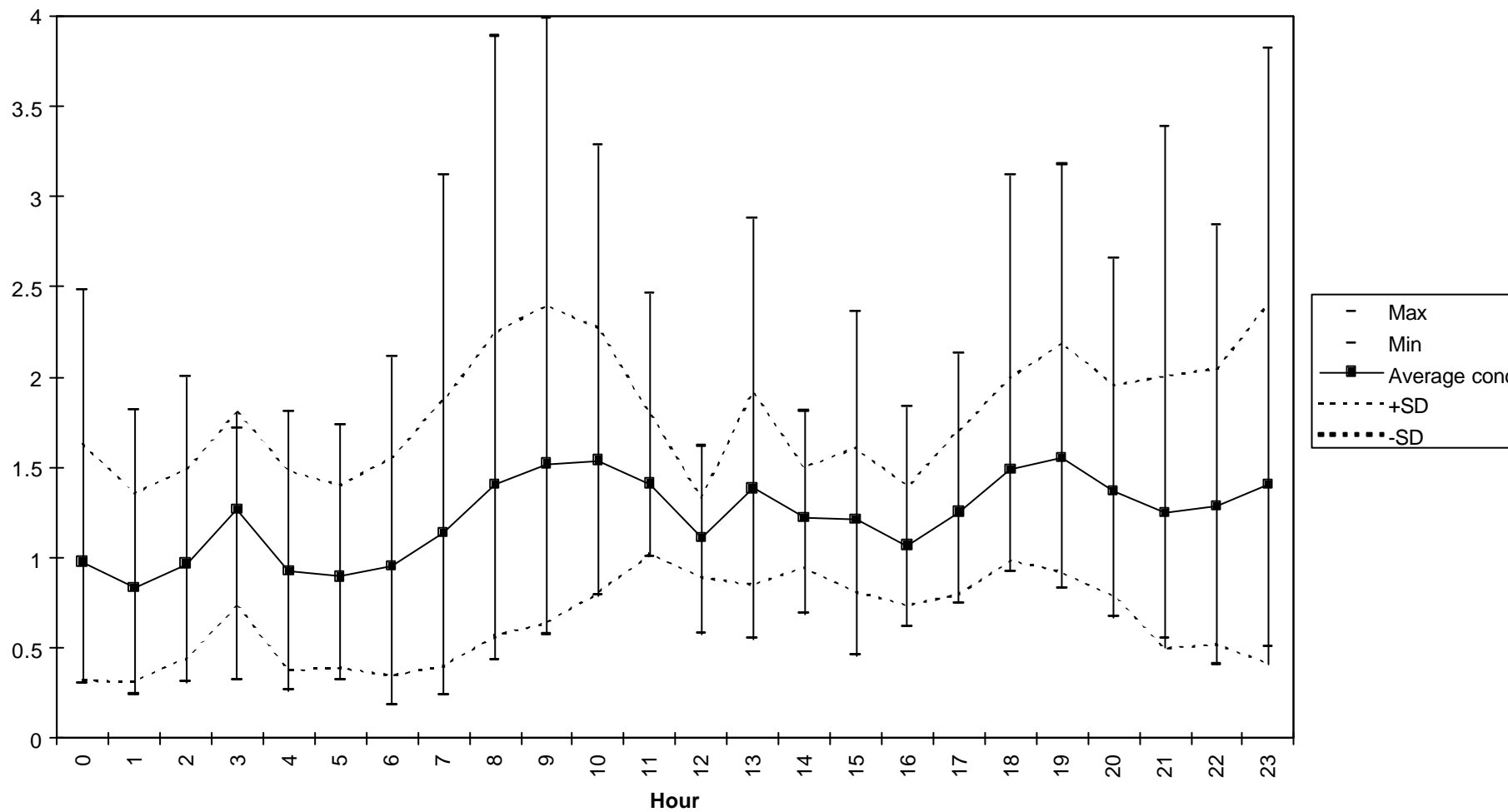
Figure 17 - Diurnal variation in formaldehyde measurements at Rochester.
