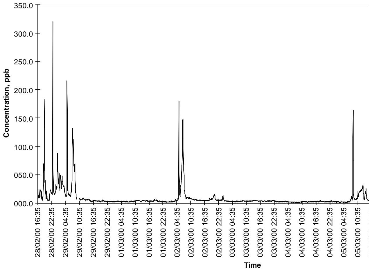
Figure 55 Time series of SO 2 measurements at an industrial site.
