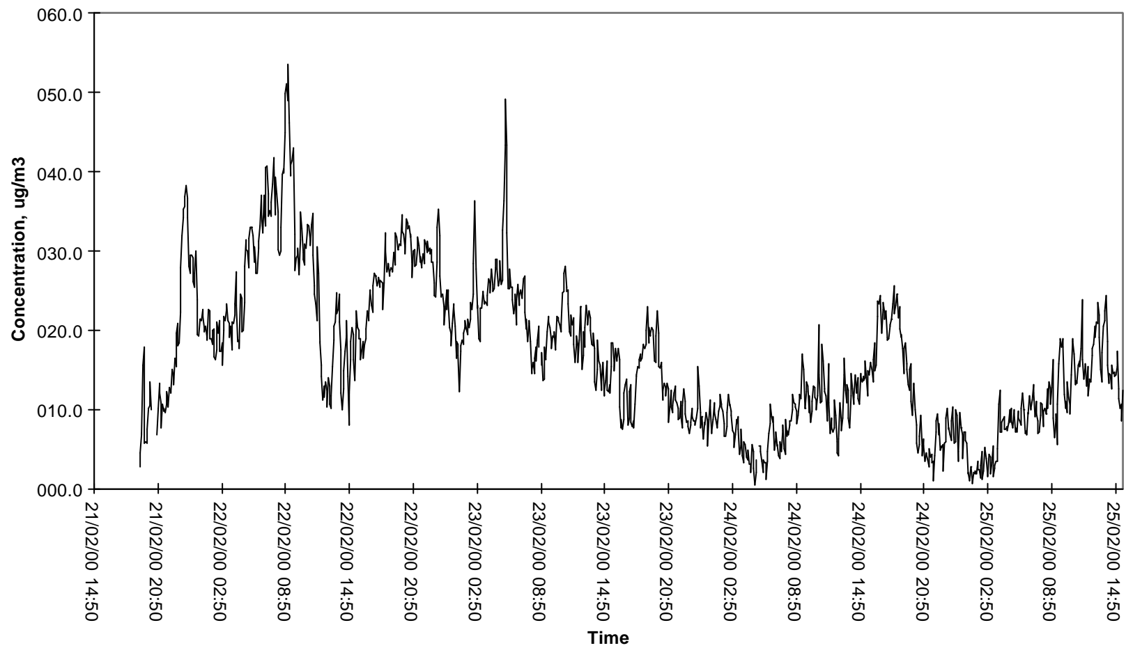
Figure 46 - Time series of PM10 measurements at Rochester.
