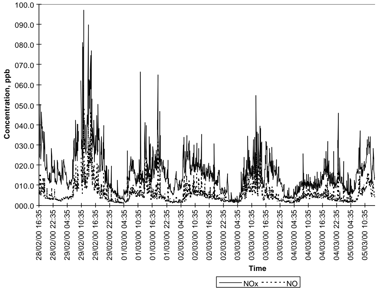
Figure 52 Time series of NO x /NO measurements at an industrial site.
