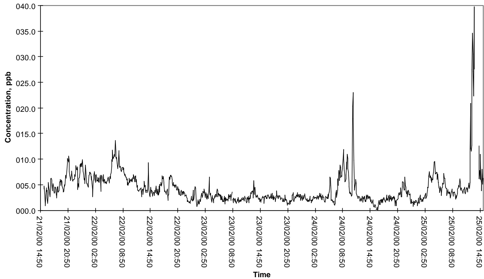
Figure 44 - Time series of SO 2 measurements at Rochester.
