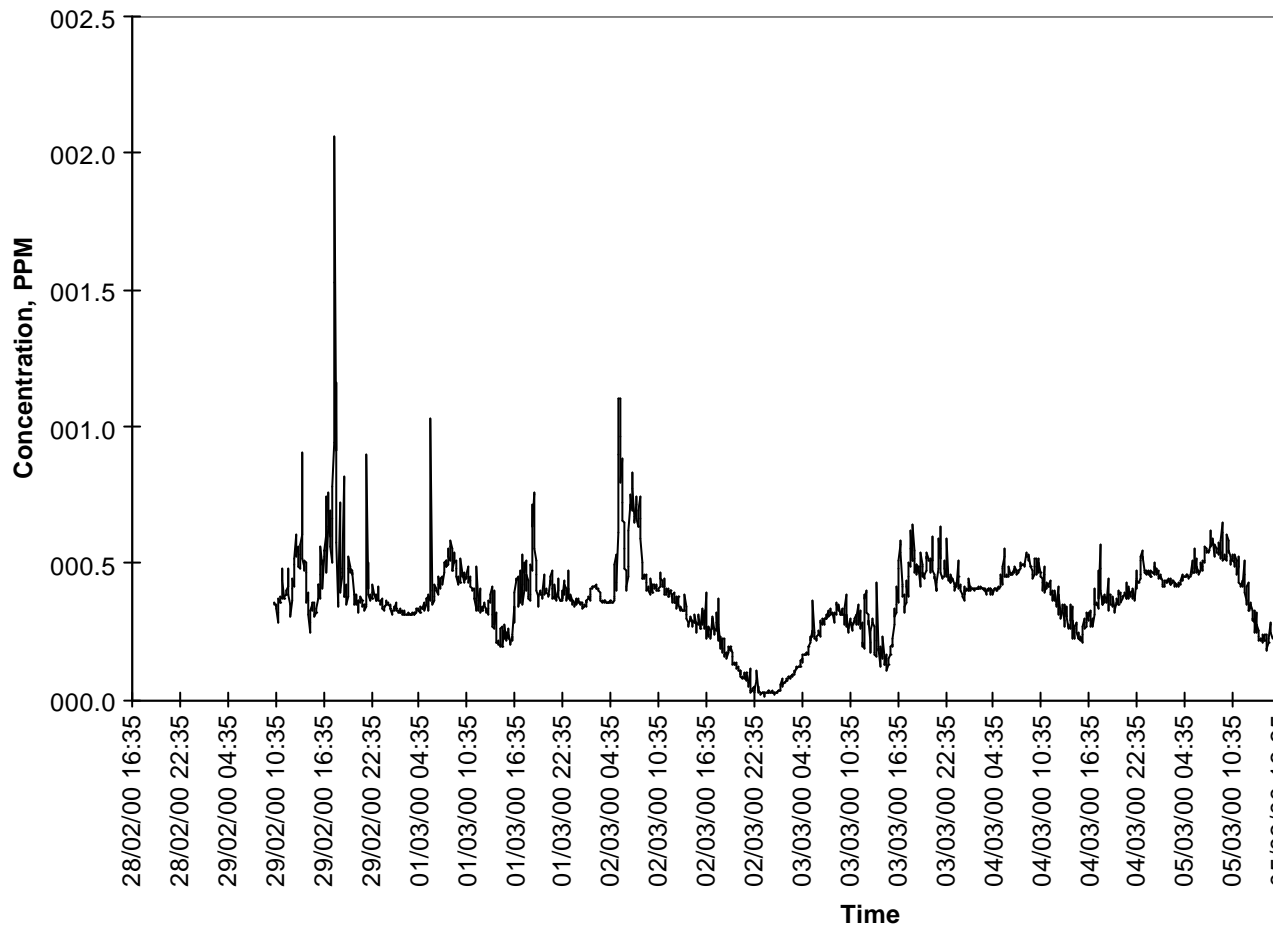
Figure 56 ime series of CO measurements at an industrial site.
