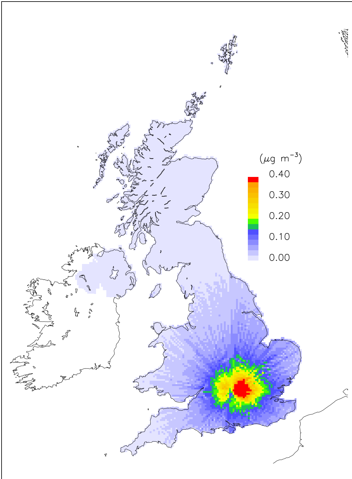
Figure 6.4: Didcot power station footprint of SO 2 simulated by the modified model with the plume distributed over four vertical layers but allowed to rise above the mixed layer into the free troposphere.
