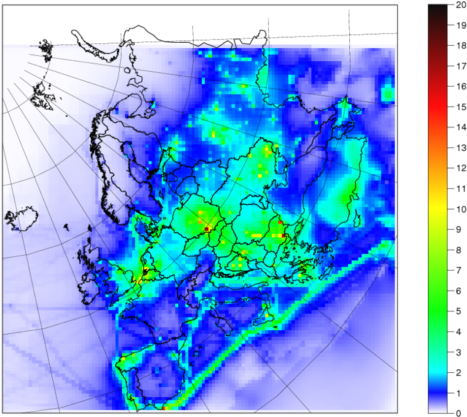
Fig. 73(f) EMEP SO 2 concentration (µg m -3 )
