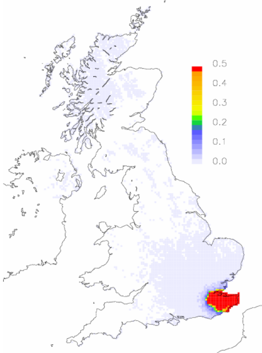
Figure 5(b) NH 3 dry deposition from Kent for 2003 (Kg N Ha -1 )
