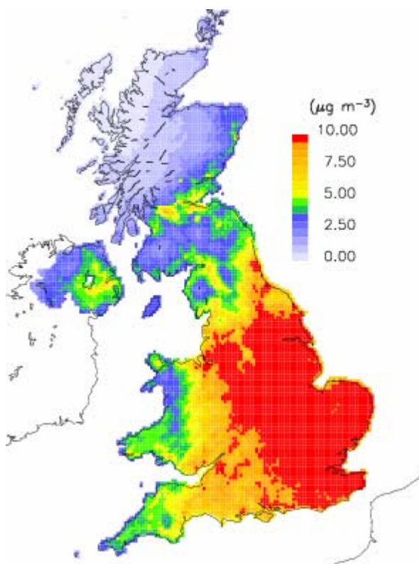
Figure 9.3 Total inorganic (primary and secondary) PM 10 concentrations ( \mu\text{g m}^{-3} )
