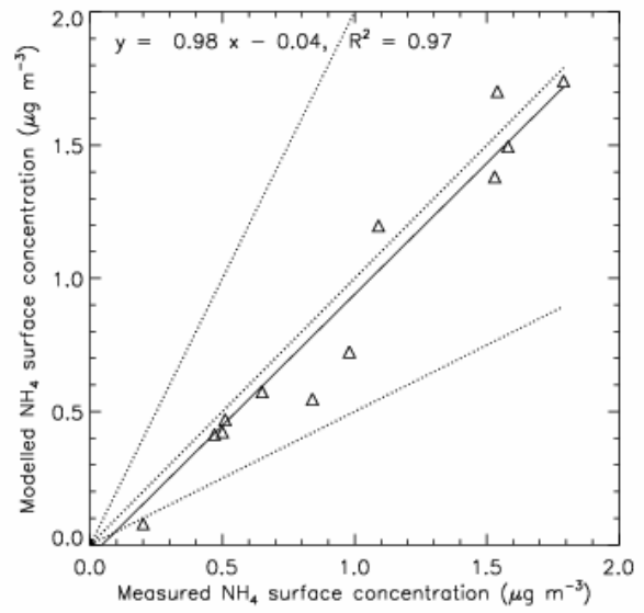
Fig. 4(f) Modelled \text{NH}_4^+ concentration correlation with measurements
