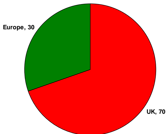
Fig. 7.4(e) FRAME source allocation for \text{NH}_x deposition in the UK
