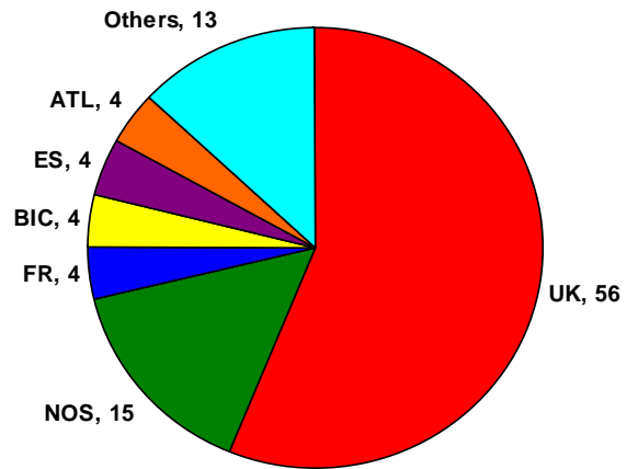
Fig. 7.4(b) EMEP source allocation for \text{SO}_x deposition in the UK
