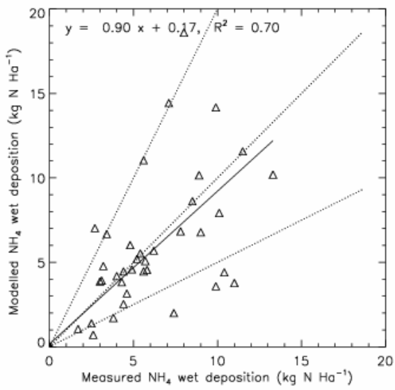
Fig. 4(h) Modelled \text{NH}_4^+ wet deposition correlation with measurements
