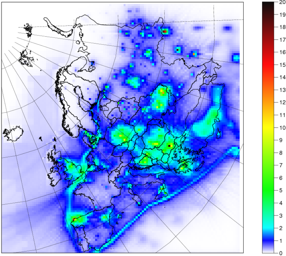
Fig. 7.3(e) FRAME-Europe SO 2 concentration (µg m -3 )
