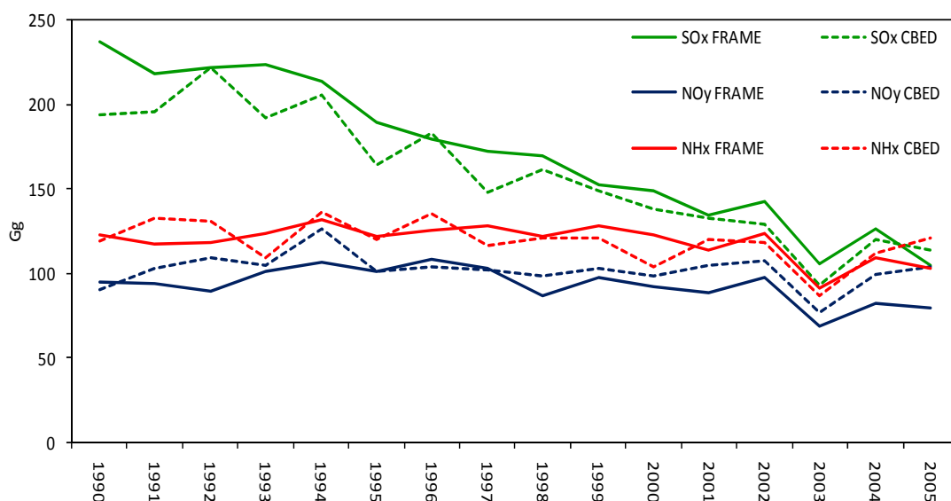
Figure 10.3 Modelled and measured UK national wet deposition budget for: S-SO x , N-NO y , N NH x (Gg).
