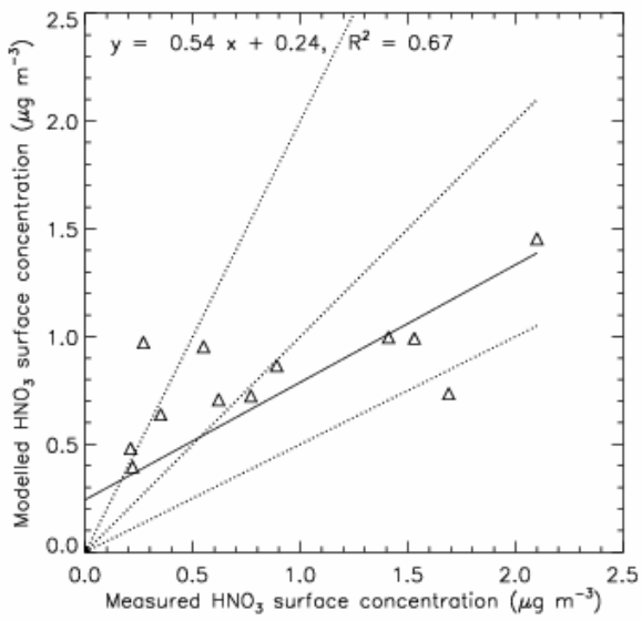
Fig. 4(g) Modelled \text{HNO}_3 concentration correlation with measurements
