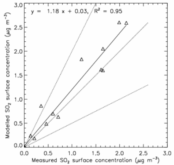
Fig. 4(b) Modelled \text{SO}_4^- concentration correlation with measurements
