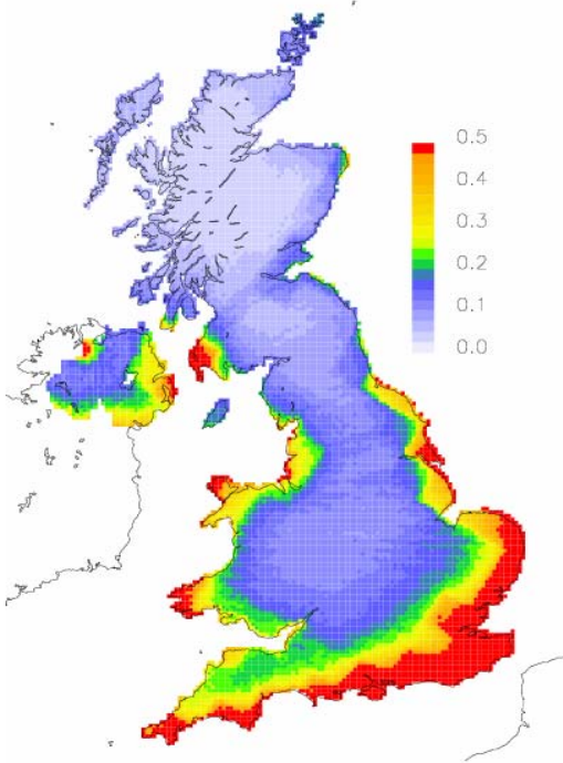
Figure 5(a) SO 2 dry deposition from shipping for 2003 (Kg S Ha -1 )
