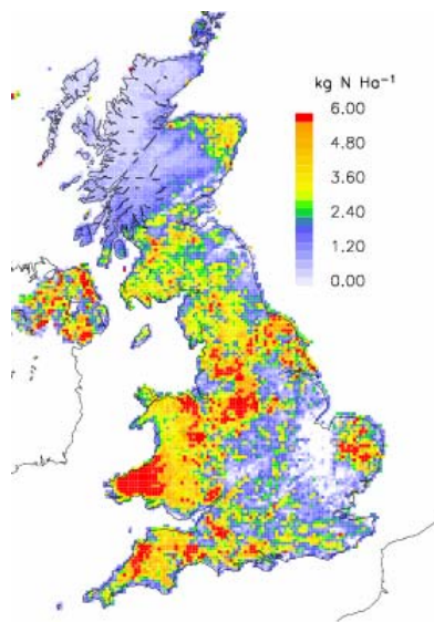
Fig. 3.3(e) CBED 2004-6 NH x dry deposition [kg N ha -1 yr -1 ]
