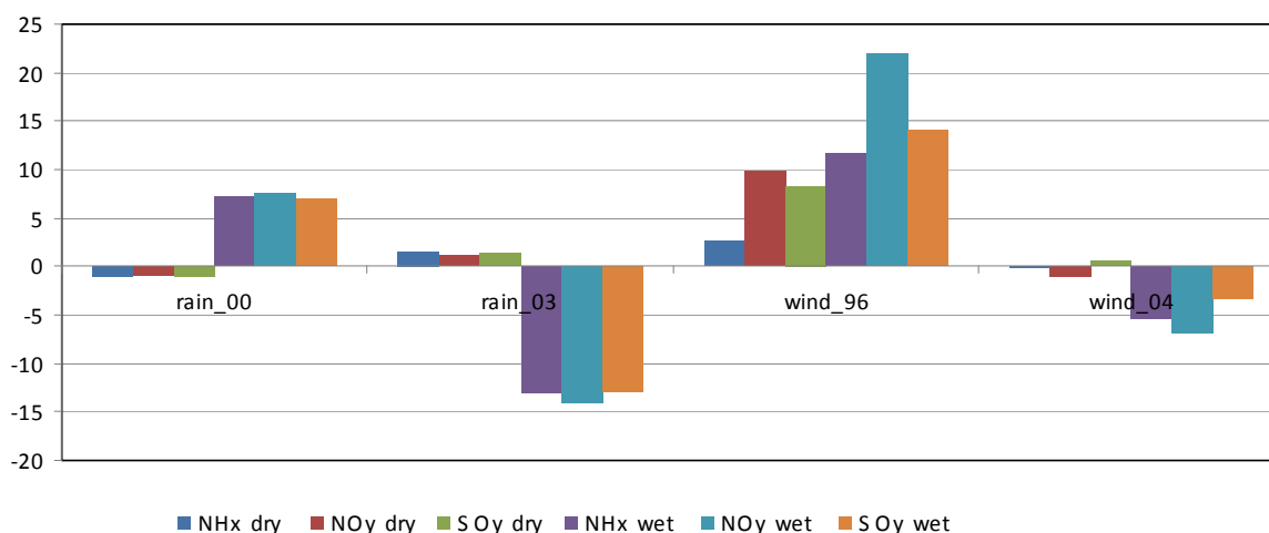
Figure 12.1: The percentage change in wet and dry deposition of sulphur and nitrogen in the UK using meteorology from the wettest (2000) and driest (2003) years and with enhanced south-easterly flow (1996) and westerly flow (2004).
