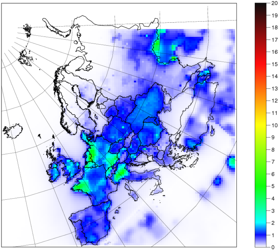
Fig. 7.3(b) EMEP NH 3 concentration (µg m -3 )
