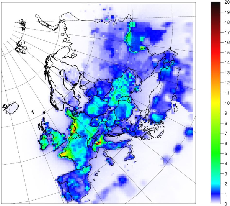
Fig. 7.3(a) FRAME-Europe NH 3 concentration (µg m -3 )
