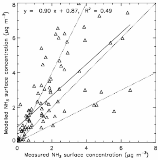
Fig. 4(e) Modelled \text{NH}_3 concentration correlation with measurements
