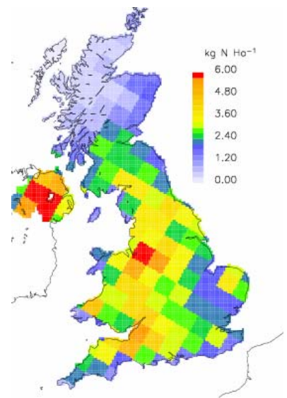
Fig. 3.3(f) EMEP 2005 NH x dry deposition [kg N ha -1 yr -1 ]
