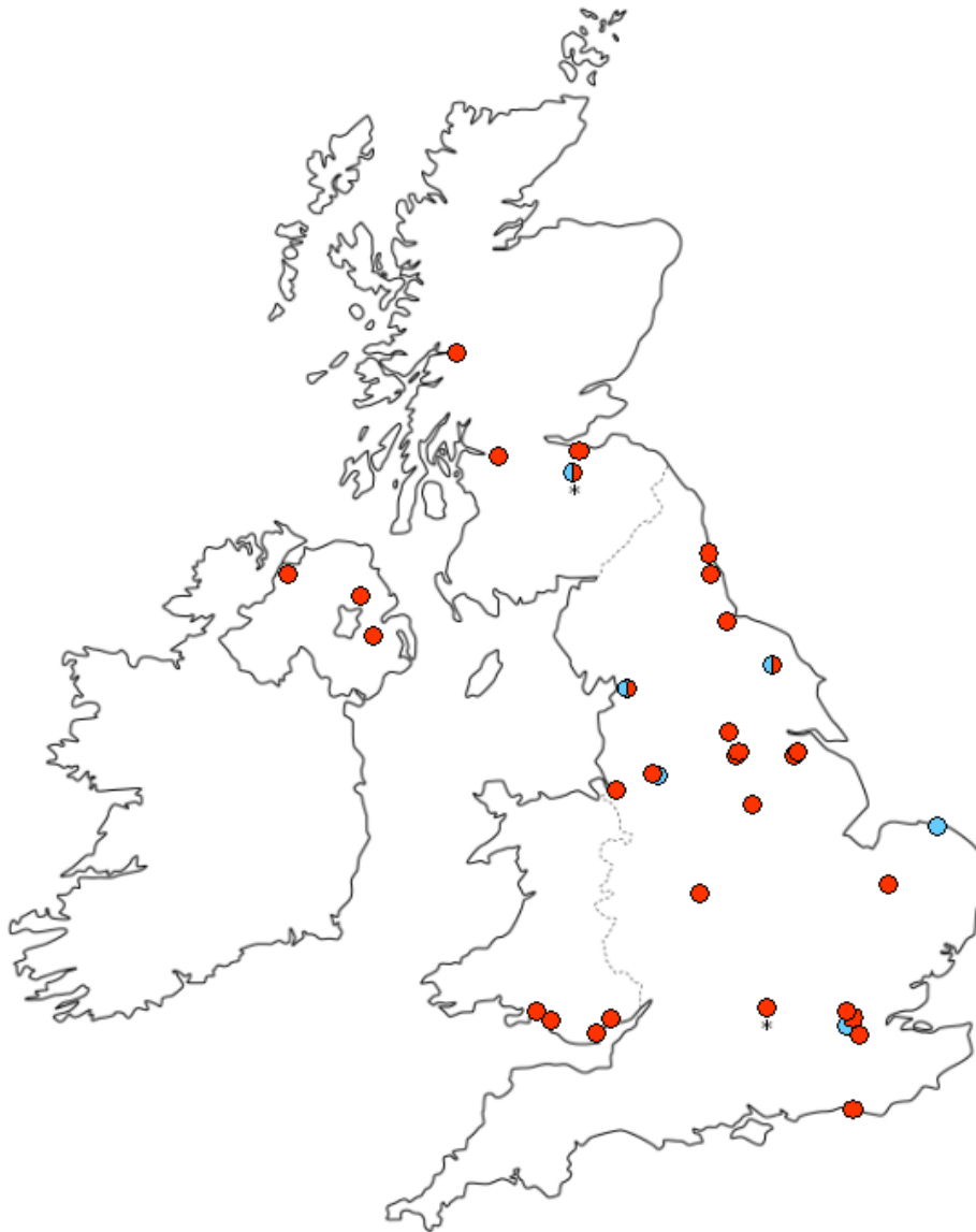
Figure 3 Schematic map showing the location of the Network stations (red circles) and TOMPS Network stations (blue circles). Co-located PAHs & TOMPs stations are shown by a half blue / half red circle. The two stations marked with asterisks are Auchencorth Moss and Harwell, where Digital particulate and vapour samples and deposition samples are also taken (see Section 3.2.2).
