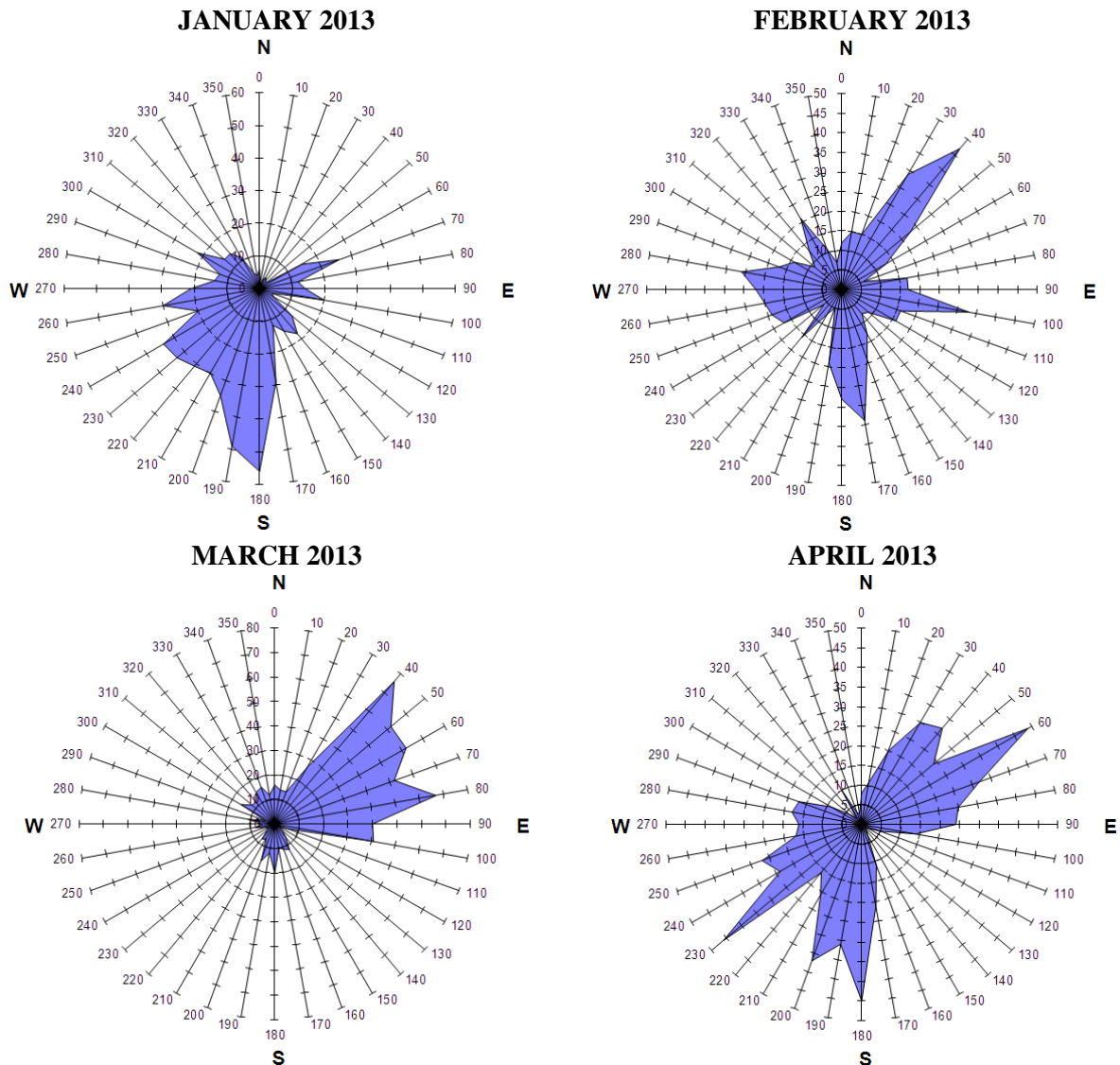
Figure 15 Wind data from the Scunthorpe Town station from January to April 2013 [27]. The average wind speed and direction recorded for each month was respectively 1 \text{ m}\cdot\text{s}^{-1} at 210^\circ , 0.5 \text{ m}\cdot\text{s}^{-1} at 47.8^\circ , 2.5 \text{ m}\cdot\text{s}^{-1} at 71.4^\circ and 0.2 \text{ m}\cdot\text{s}^{-1} at 132.9^\circ .
