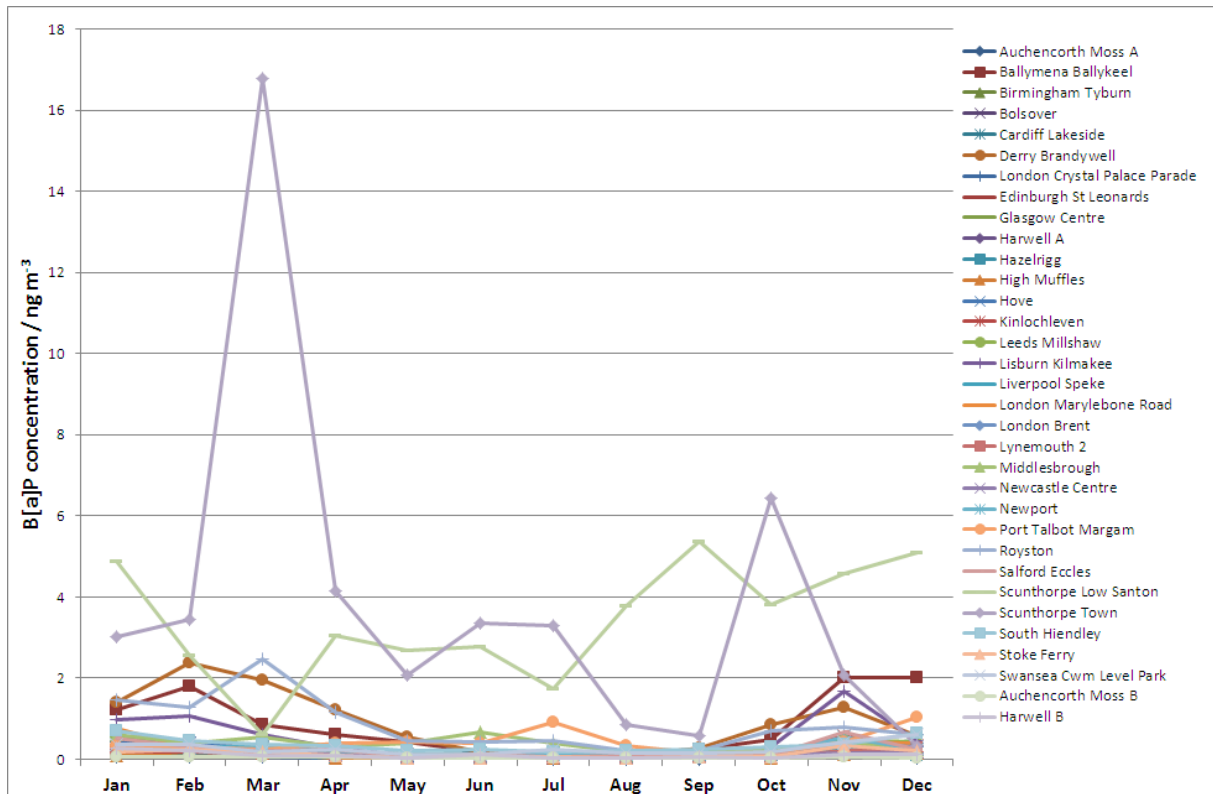
Figure 10 Monthly mean B[a]P concentrations recorded at ‘A’ and ‘B’ stations during 2013
