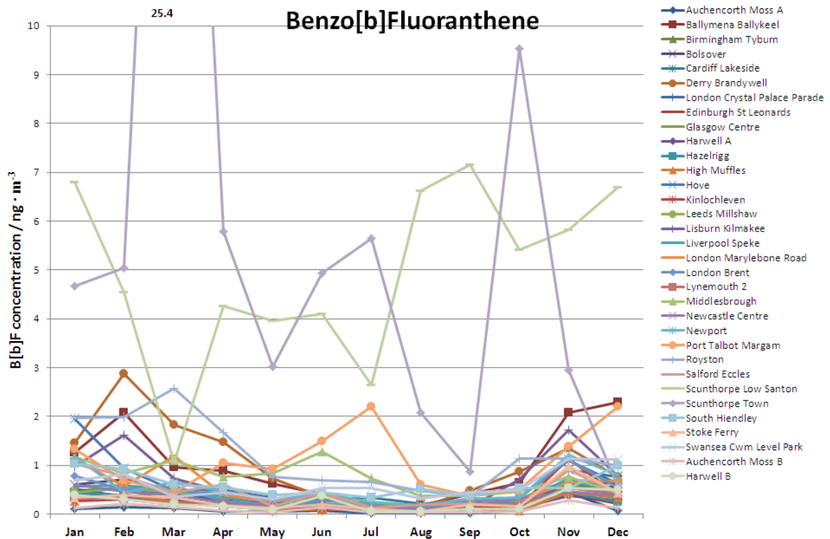
Figure 12(b) Monthly mean benzo[b]fluoranthene concentrations recorded at ‘A’ and ‘B’ stations during 2013
