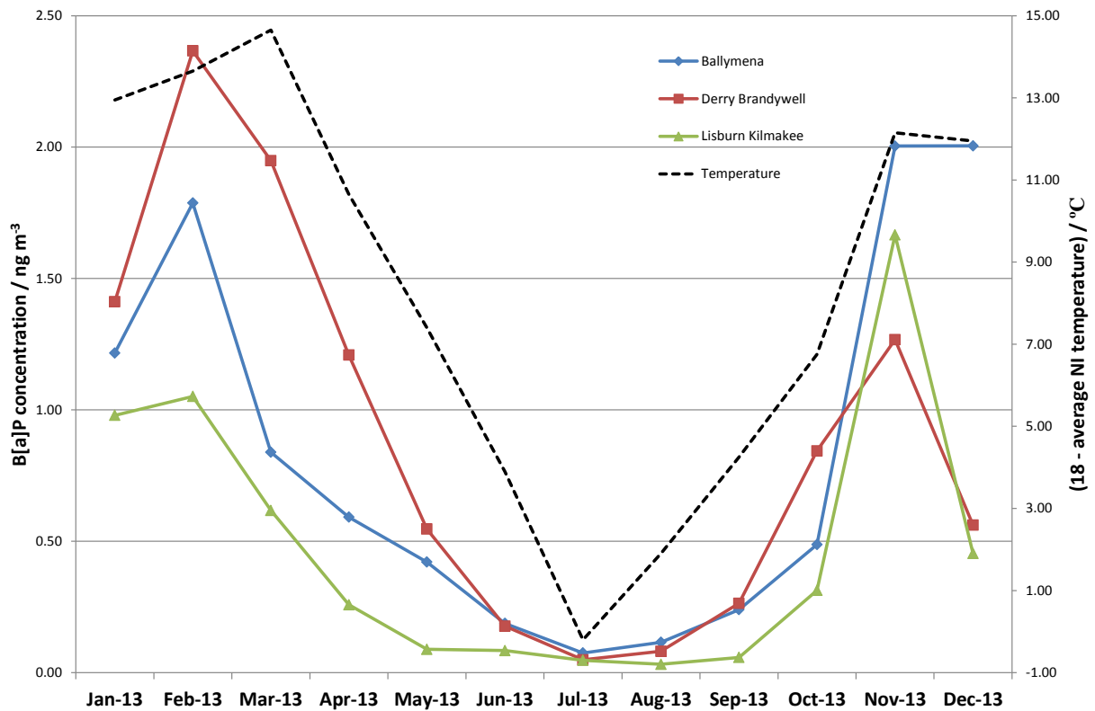
Figure 11(a) Monthly mean B[a]P concentrations recorded at background / urban stations in Northern Ireland during 2013, plotted together with the 2013 monthly average temperature (plotted as (18 - T) ^\circ\text{C} )
