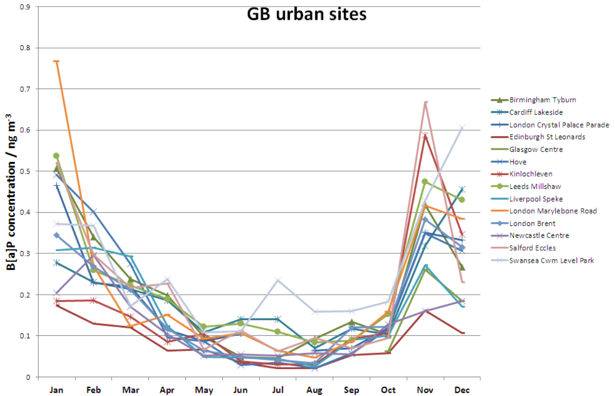
Figure 11(b) Monthly mean B[a]P concentrations recorded during 2013 at the traffic / urban (London Crystal Palace Parade and London Marylebone Road) and background / urban stations in Great Britain not influenced by major industrial processes (all others).
