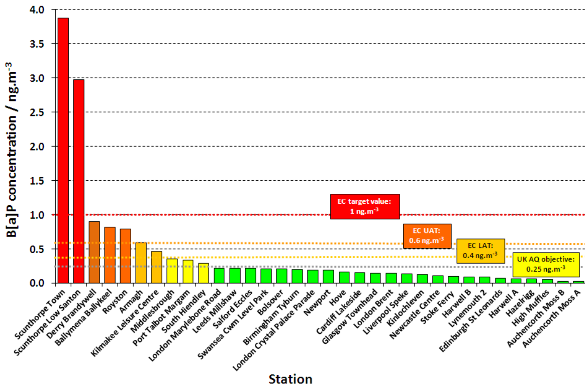
Figure 9 Annual mean B[a]P concentrations recorded at 'A' and 'B' stations during 2013. (Note: Glasgow Townhead runs for the period 16 Oct – 31 Dec). The colour coding of the data from each station indicates that the mean concentration is:
