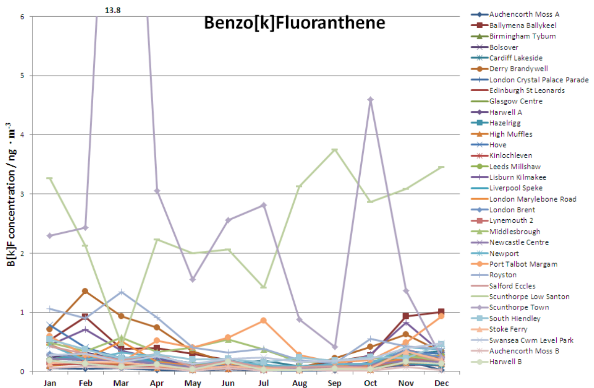
Figure 12(d) Monthly mean benzo[k]fluoranthene concentrations recorded at ‘A’ and ‘B’ stations during 2013
