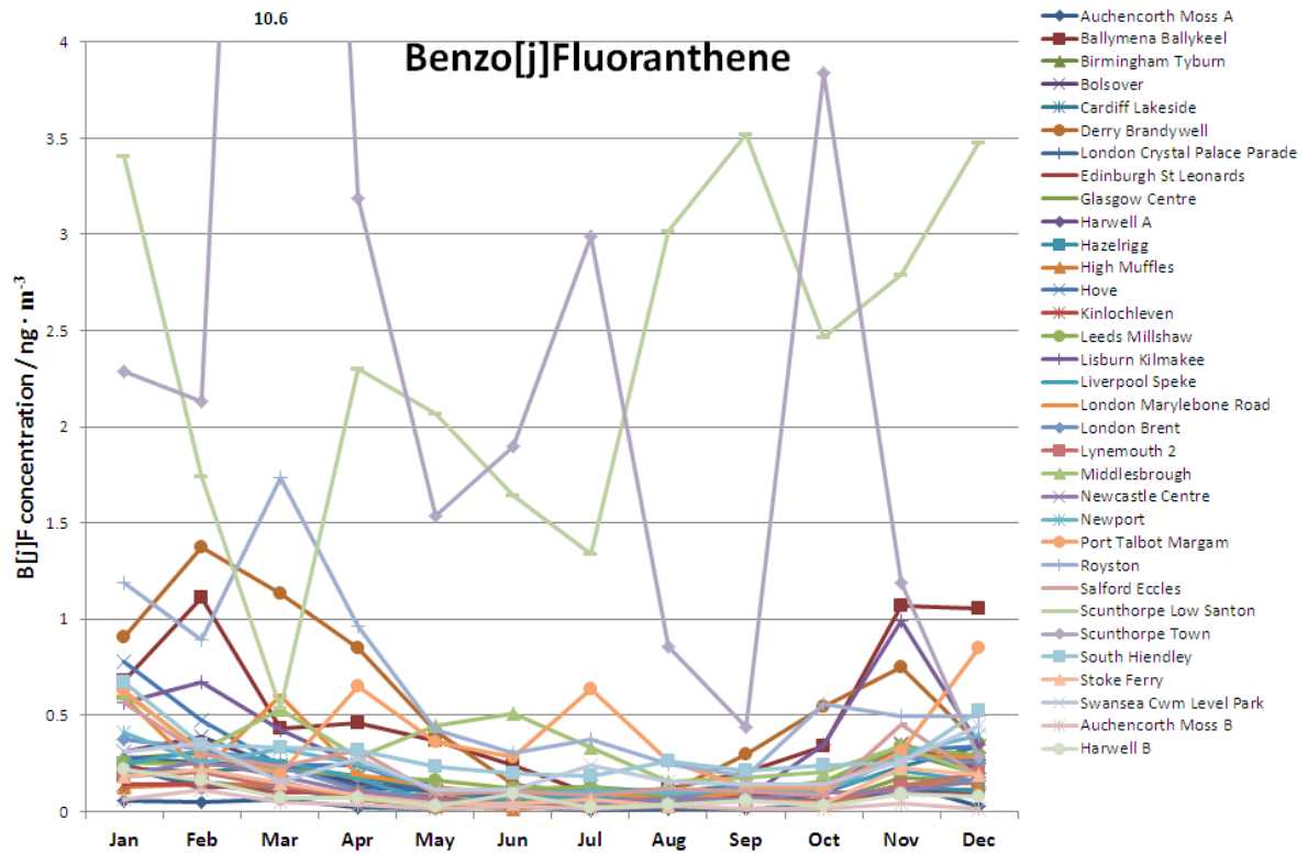
Figure 12(c) Monthly mean benzo[j]fluoranthene concentrations recorded at ‘A’ and ‘B’ stations during 2013
