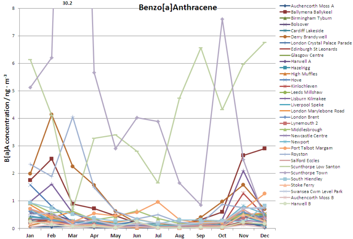
Figure 12(a) Monthly mean benz[a]anthracene concentrations recorded at ‘A’ and ‘B’ stations during 2013
