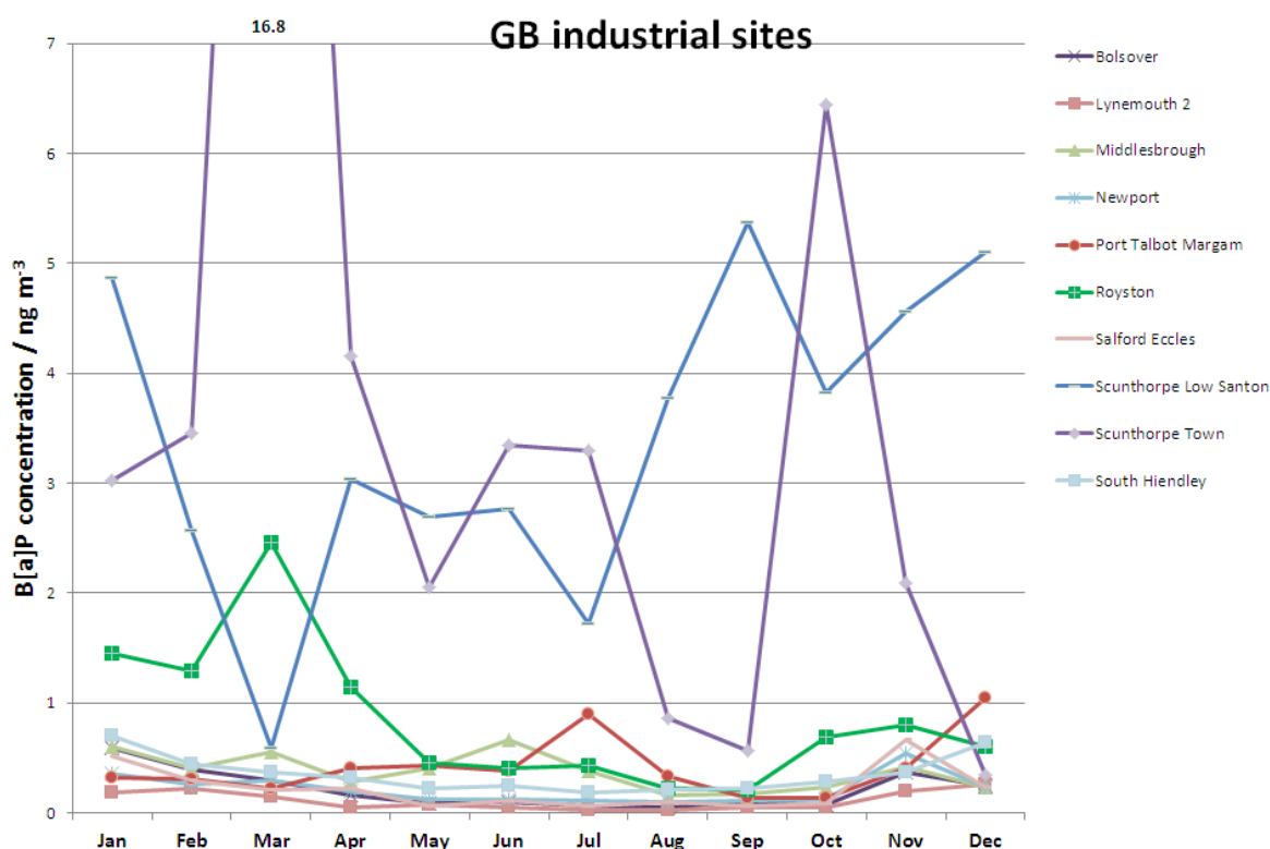
Figure 11(d) Monthly mean B[a]P concentrations recorded during 2013 at Network stations influenced by major industrial processes. The stations are: five industrial / urban stations (Middlesbrough, Port Talbot Margam, Royston, Scunthorpe Low Santon, Scunthorpe Town & South Hiendley), one industrial / suburban station (Lynemouth 2) and three background / urban stations in Great Britain that are influenced by industrial plants (Bolsover, Salford Eccles & Newport)
