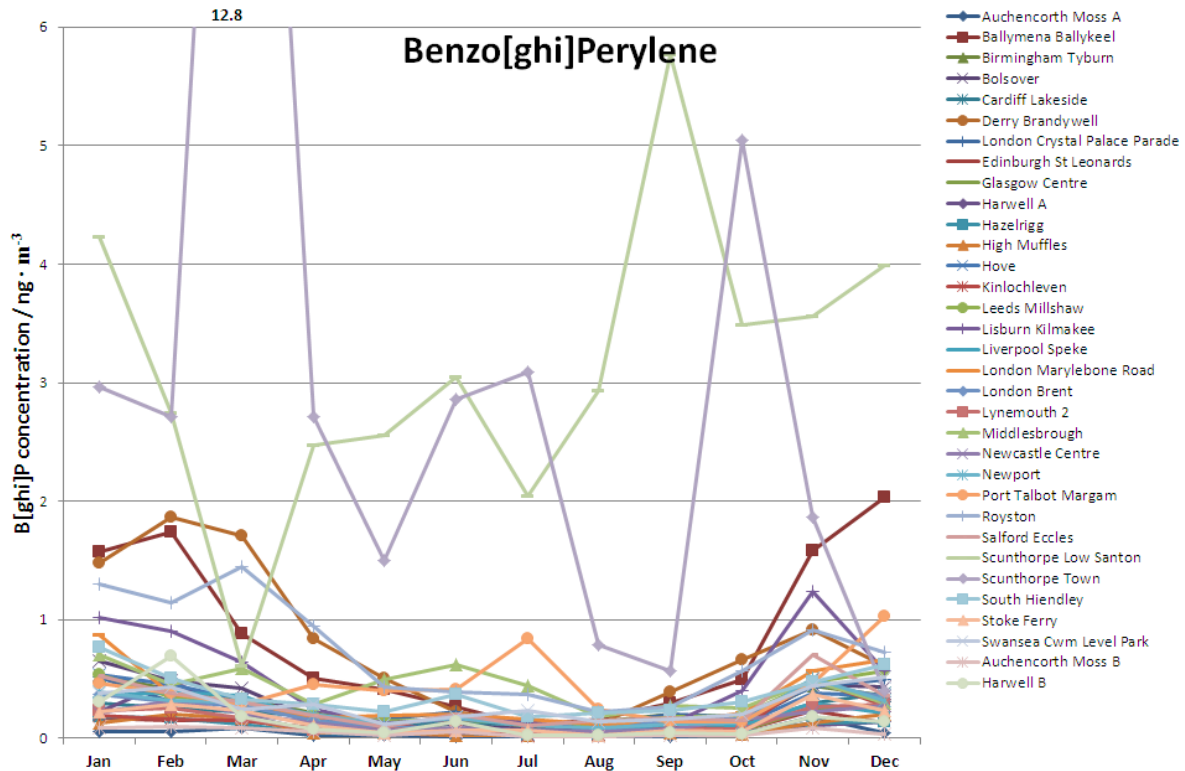
Figure 12(g) Monthly mean benzo[ghi]perylene concentrations recorded at ‘A’ and ‘B’ stations during 2013
