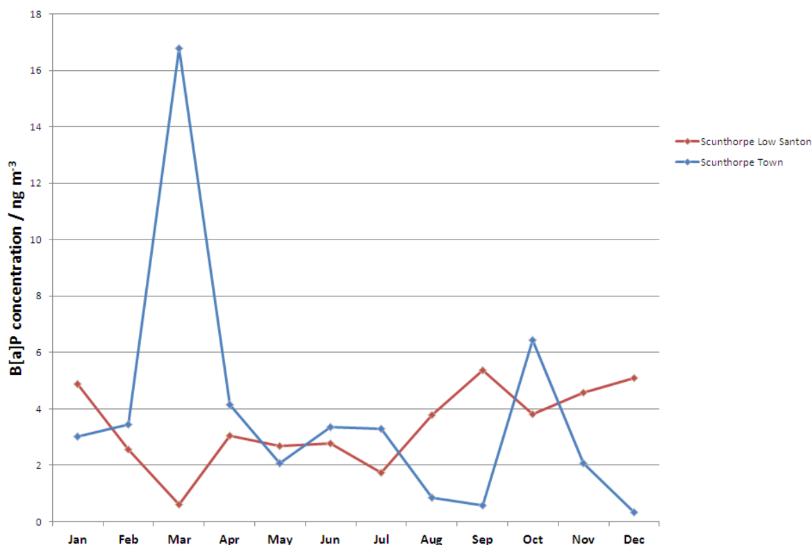
Figure 13 Monthly mean B[a]P concentrations recorded during 2013 at Scunthorpe Low Santon and Scunthorpe Town
