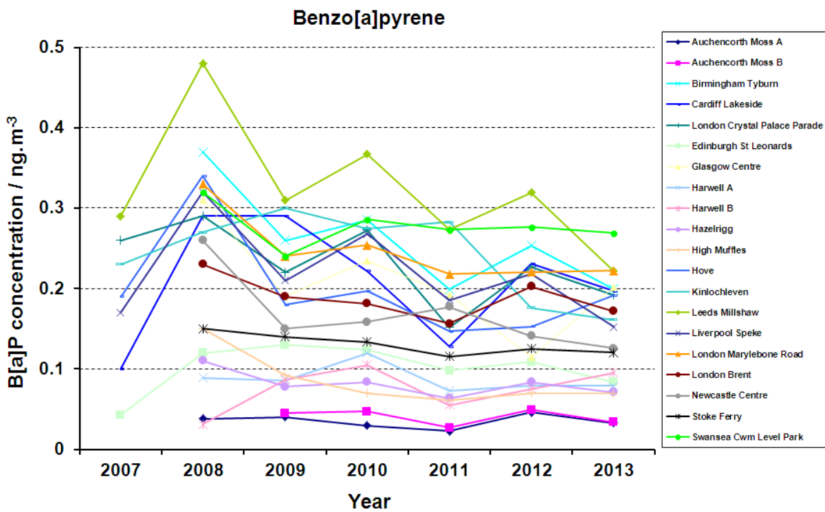
Figure 17(b) Annual mean B[a]P concentration measured at all ‘A’ & ‘B’ stations (except all stations in Northern Ireland, and those stations in Great Britain influenced by major industrial processes) from 2007-2013 inclusive
