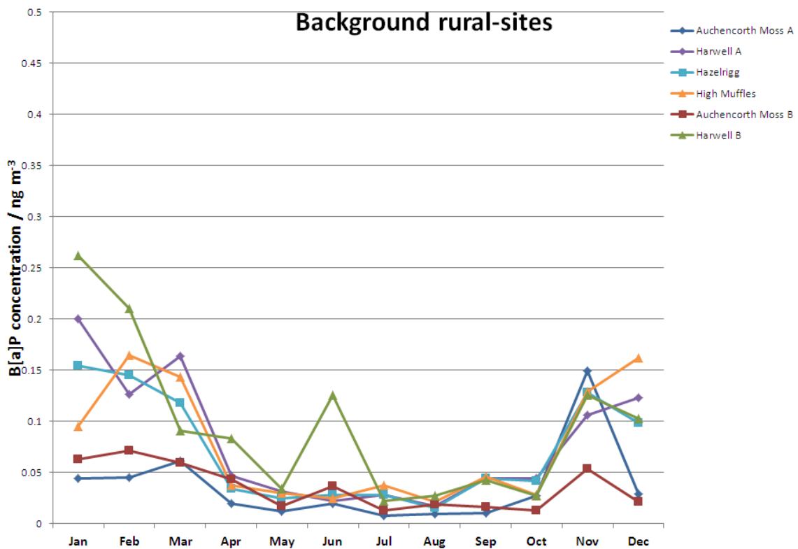
Figure 11(c) Monthly mean B[a]P concentrations recorded during 2013 at background / rural stations
