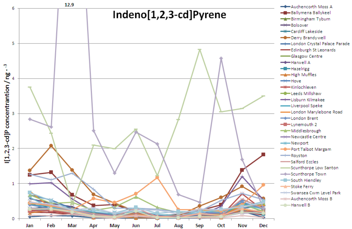
Figure 12(e) Monthly mean indeno[1,2,3-cd]pyrene concentrations recorded at ‘A’ and ‘B’ stations during 2013
