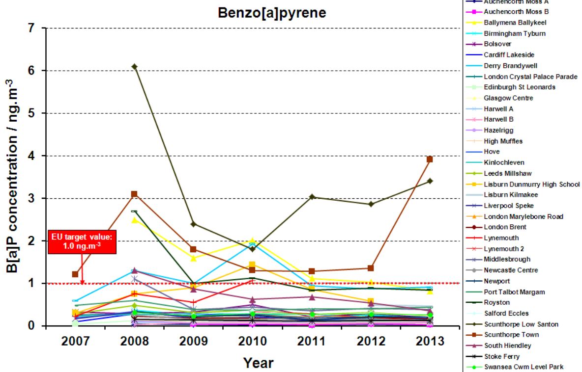
Figure 17(a) Annual mean B[a]P concentration measured at all ‘A’ & ‘B’ stations from 2007-2012/3 inclusive
