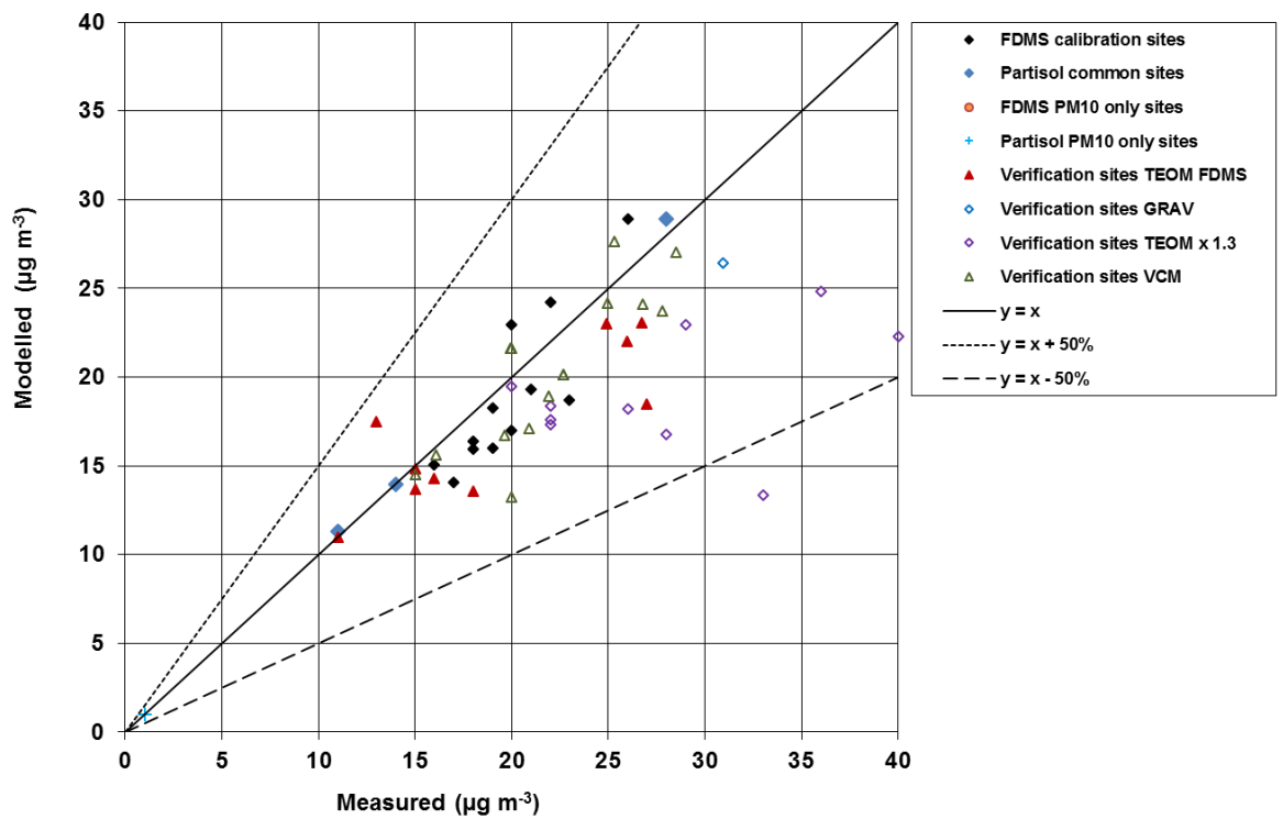
Figure 5.10 - Verification of roadside annual mean PM 10 model 2014
