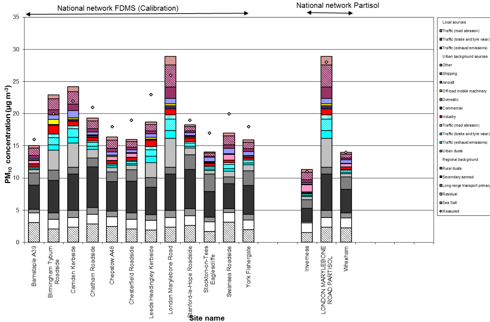
Figure 5.12 - Annual mean PM 10 source apportionment at national network roadside monitoring sites in 2014
