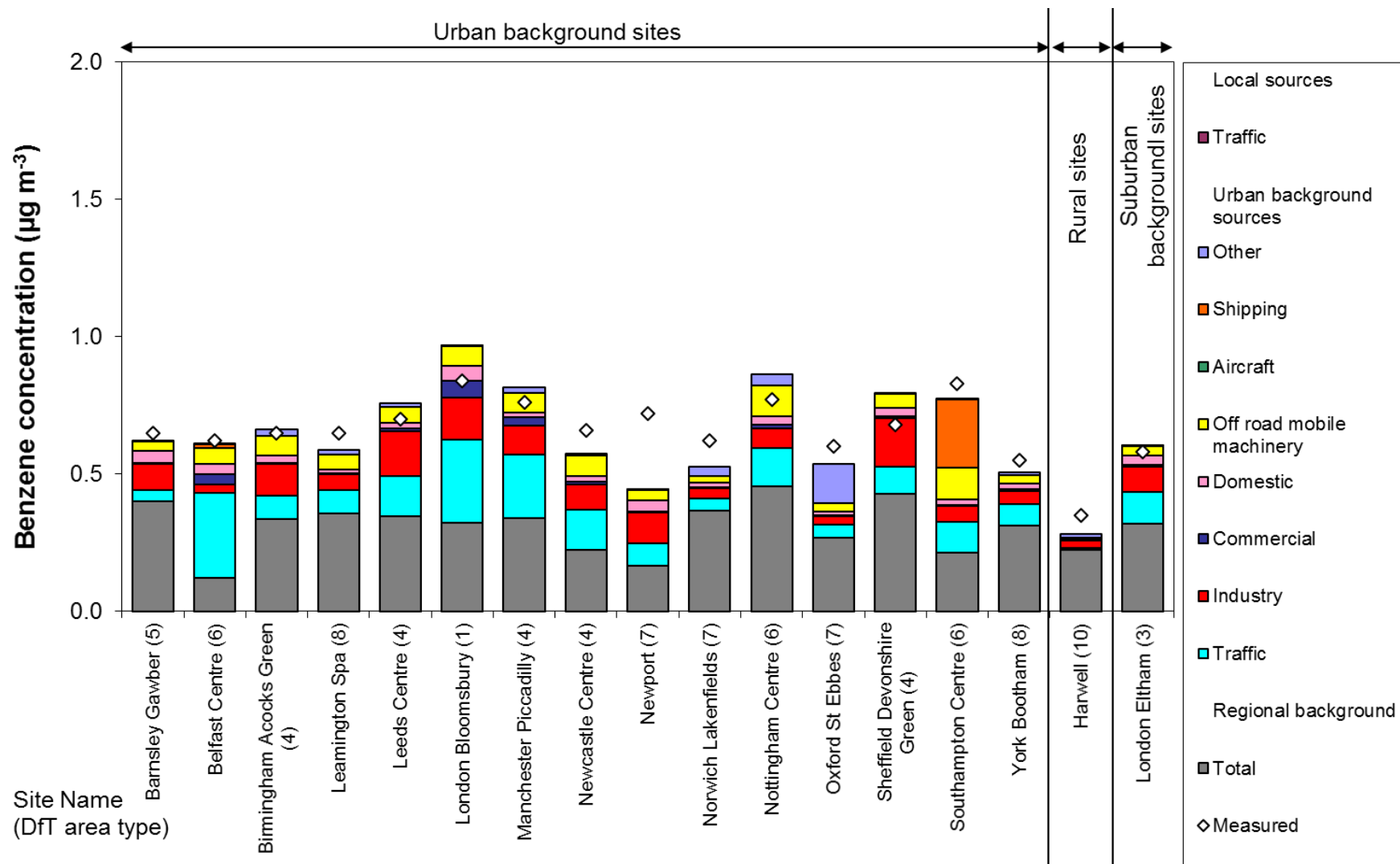
Figure 7.8 - Annual mean benzene source apportionment at background monitoring sites in 2014 (the area type of each site is shown in parenthesis after its name)
