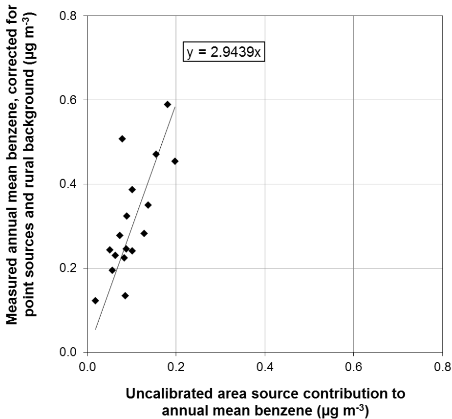
Figure 7.4 - Calibration of area source benzene model, 2014 ( \mu\text{g m}^{-3} )
