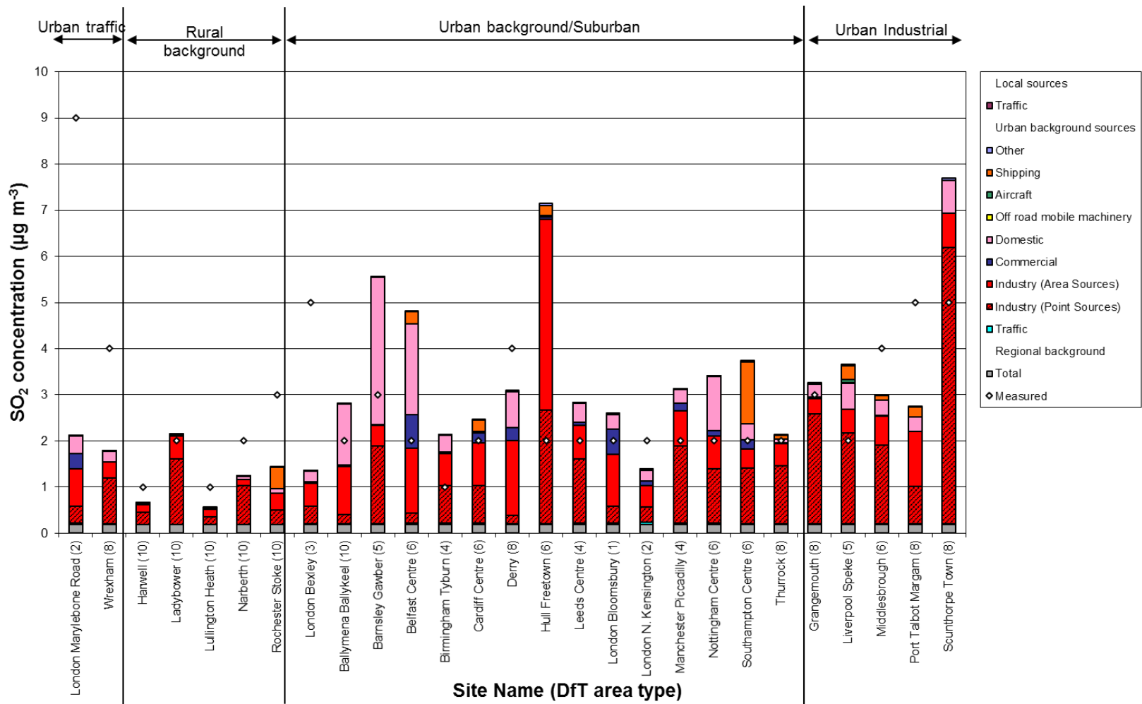
Figure 4.14 - Annual mean SO 2 source apportionment at AURN monitoring sites in 2014 (the area type of each site is shown in parenthesis after its name – see Table 3.4)
