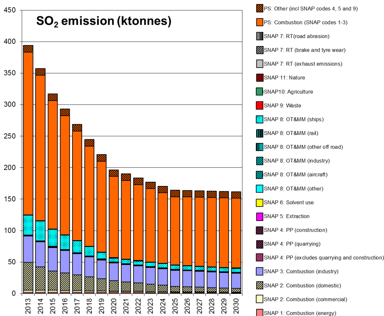
Figure 4.5 - Total UK SO 2 emissions for 2013 and emissions projections up to 2030 by SNAP code from NAEI 2013
