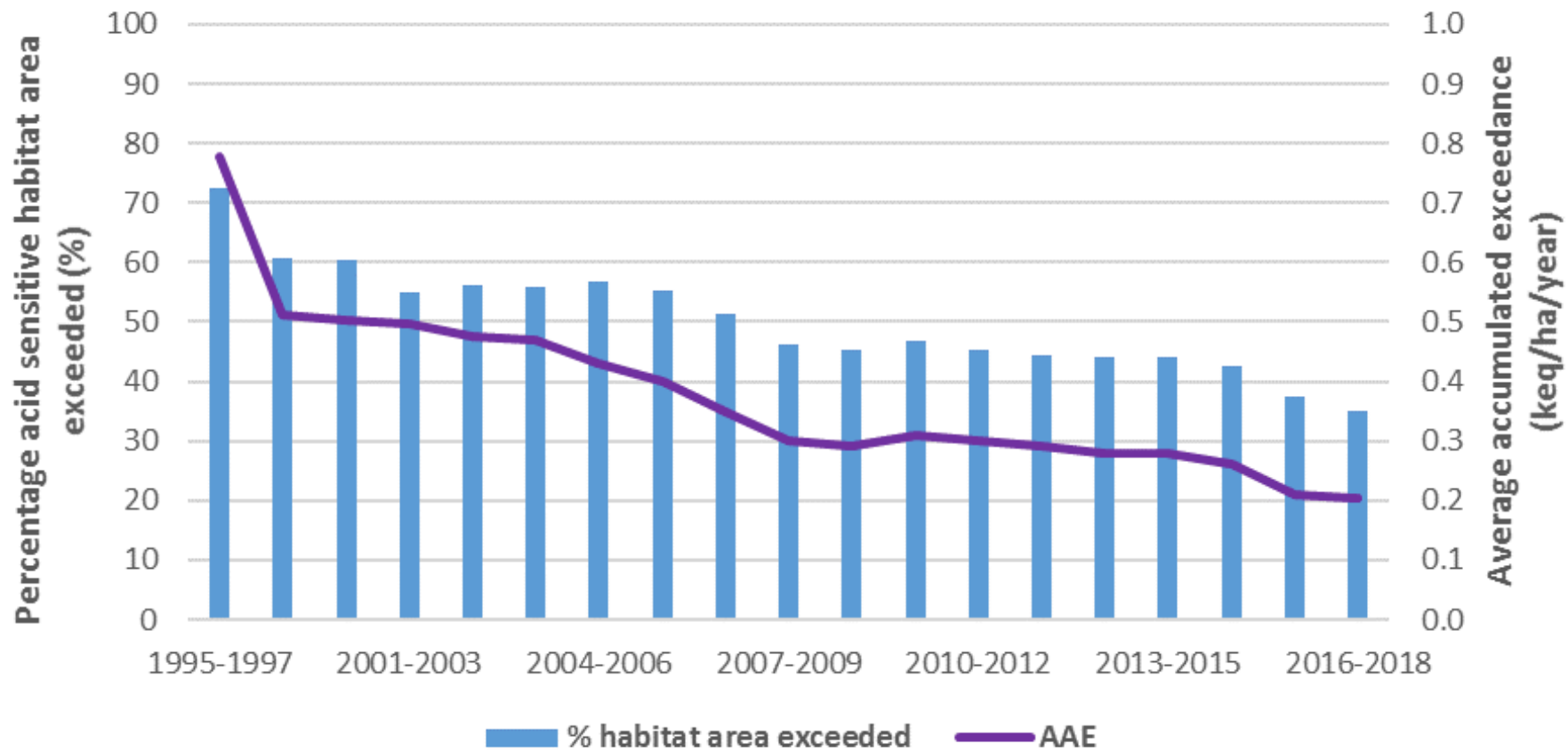
Figure 2.1: Acidity: Percentage area of acid-sensitive habitats with exceedance of acidity critical loads in the UK by year, and AAE in keq ha -1 year -1 .
