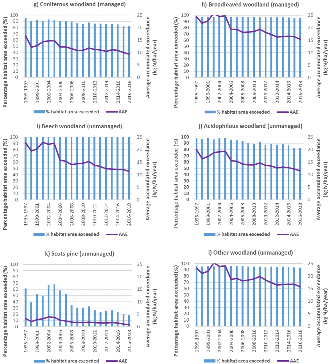
Figure 2.6 (continued): Nutrient nitrogen: Percentage area of habitats where nutrient nitrogen critical loads are exceeded and Average Accumulated Exceedance (AAE in kg N ha -1 year -1 ) i.e. “Excess Nitrogen” in the UK by deposition dataset year.
