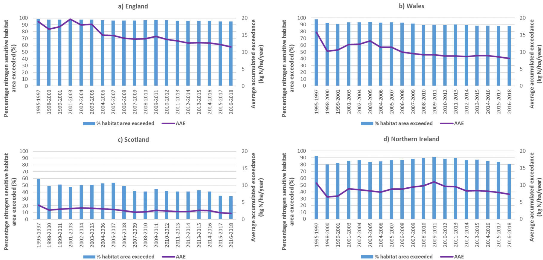
Figure 2.4: Nutrient nitrogen: Percentage area of nitrogen-sensitive habitats with exceedance of nitrogen critical loads, by country and year, and Average Accumulated Exceedance (AAE in kg N ha -1 year -1 ) i.e. “Excess Nitrogen”.
