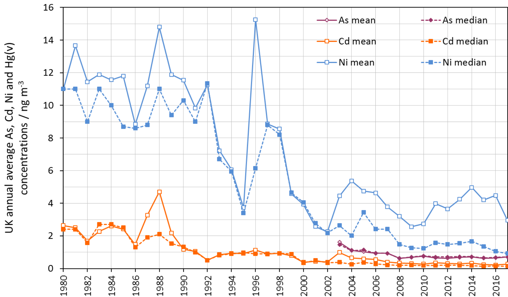
Figure 12. The mean and median of site annual average concentrations of Ni, As and Cd measured on the UK Heavy Metals Monitoring Network over the last 37 years. The EC target values for Ni, As and Cd are 20 \text{ ng m}^{-3} , 6 \text{ ng m}^{-3} and 5 \text{ ng m}^{-3} respectively.
