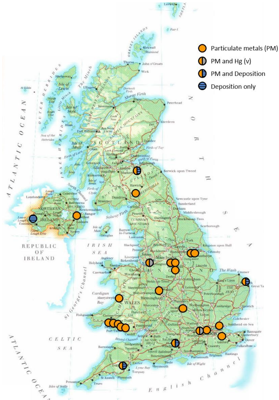
Figure A1. Location of monitoring sites comprising the UK Heavy Metals Monitoring Network during 2017 (indicated by the coloured circles, see key) – details of which are given in Table A1 below.
