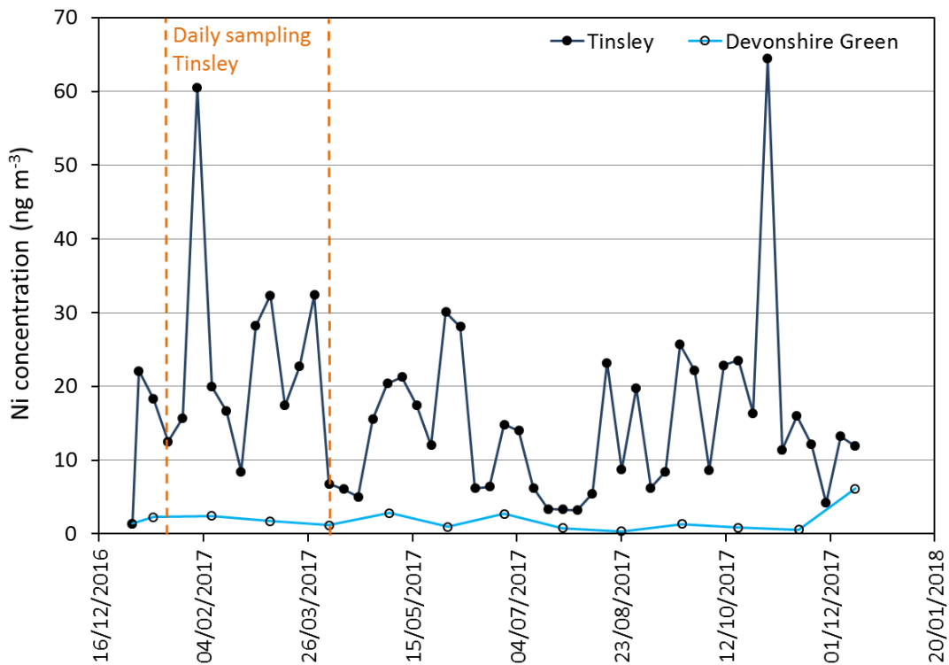
Figure 8. Measured Ni concentrations at Site 117: Sheffield Tinsley and Site 119: Sheffield Devonshire Green in 2017. Sampling at Tinsley is weekly, except for the period 18 th January – 5 th April 2017, when daily sampling was implemented. For this period weekly averages of the daily results have been plotted. Results from Sheffield Devonshire Green are averaged over 4-weekly periods.
