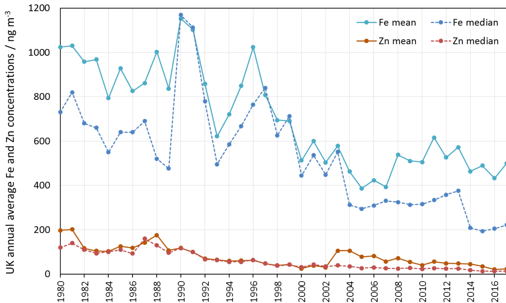
Figure 13. The mean and median of site annual average concentrations of Fe and Zn measured on the UK Heavy Metals Monitoring Network over the last 37 years.
