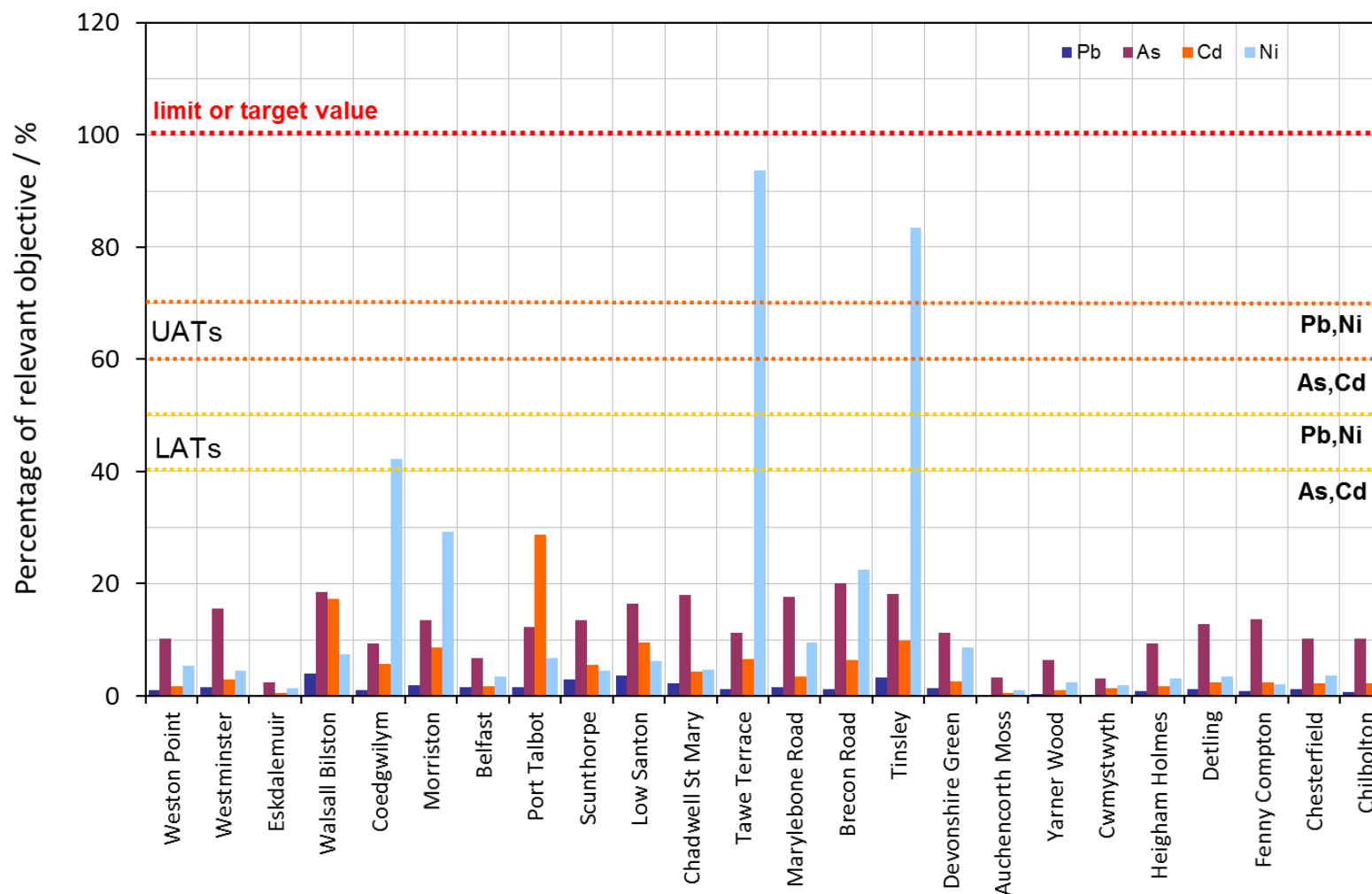
Figure 5. A summary of the annual mean measured concentrations of the heavy metals relevant to the New Air Quality Directive and Fourth DD at all sites on the UK Heavy Metals Monitoring Network in 2017 as a percentage of the relevant target values shown in red, lower assessment thresholds (LATs) in yellow and upper assessment thresholds (UATs) in orange.
