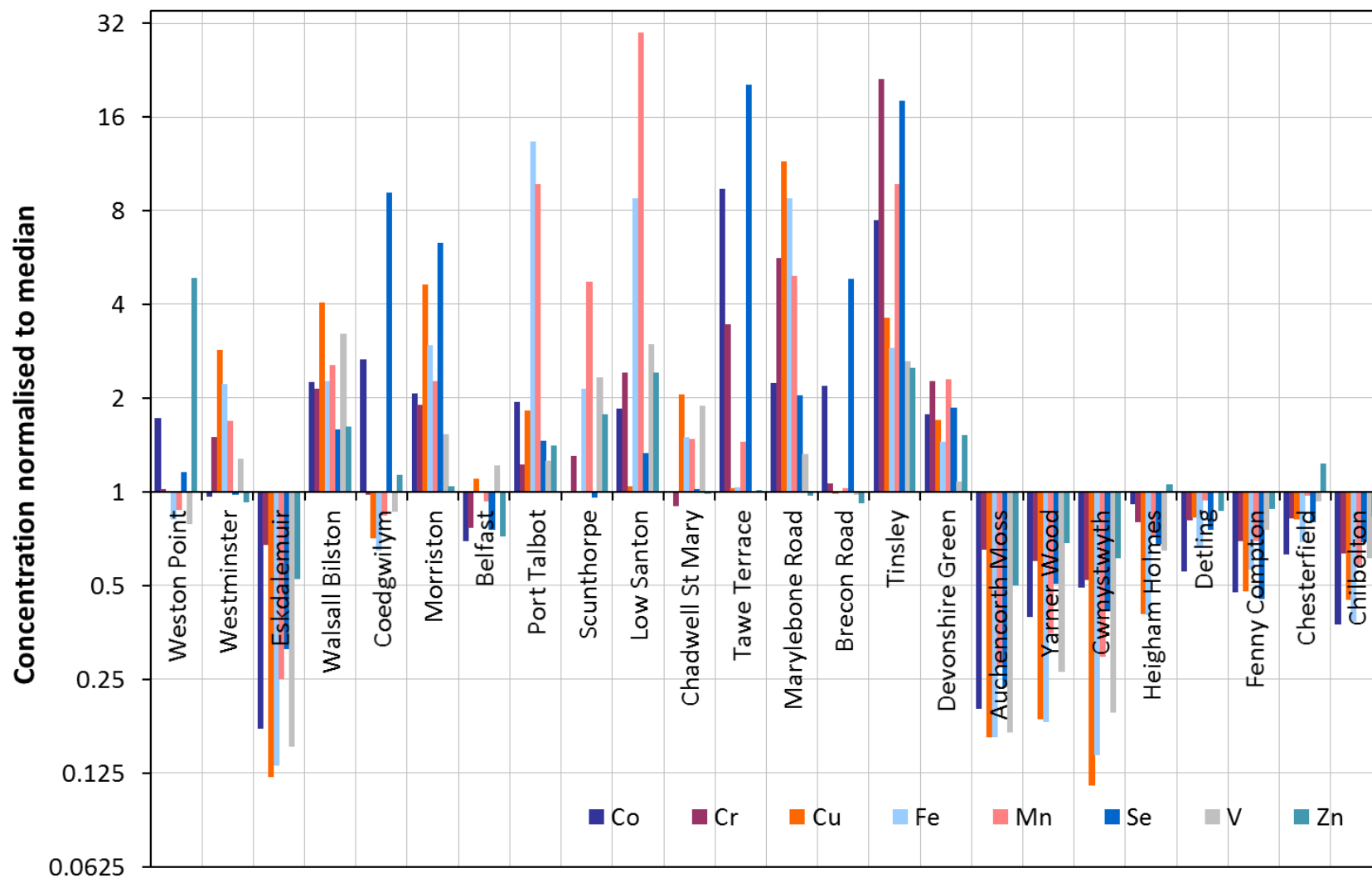
Figure 10. A summary of the annual mean measured concentrations of the non-directive metals at all sites on the UK Heavy Metals Monitoring Network in 2017, normalised to the UK annual median concentration for the relevant element. These values are plotted with respect to the median so it is clear which sites are above and below the median level. Note the logarithmic scale on the y-axis.
