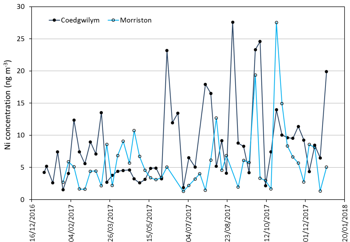
Figure 6. Measured Ni concentrations at Site 100: Swansea Coedgwilym and Site 101: Swansea Morryston, in 2017 (both sampled weekly).
