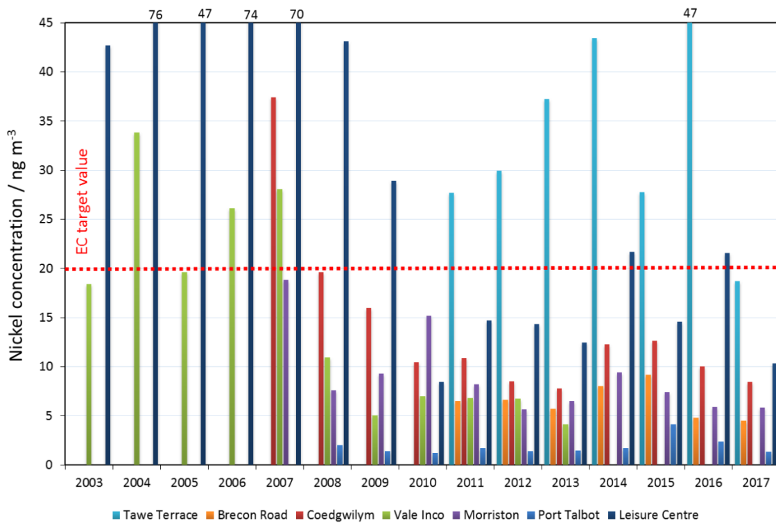
Figure 16. The annual average nickel concentrations measured at monitoring sites in the Swansea area (indicated by the key) 2003 - 2017. Nickel concentrations at Port Talbot (since monitoring began in 2008) have also been included to indicate the regional background level. The red dotted line indicates the Fourth DD target value for nickel. (The data for Vale Inco in 2008 – 2013, and Coedgwilym and Morryston in 2007 are courtesy of the City and County of Swansea. The data for the Leisure Centre is courtesy of Neath Port Talbot County Borough Council.) Note: the Vale Inco data for 2013 was only based on 18.8% data capture.
