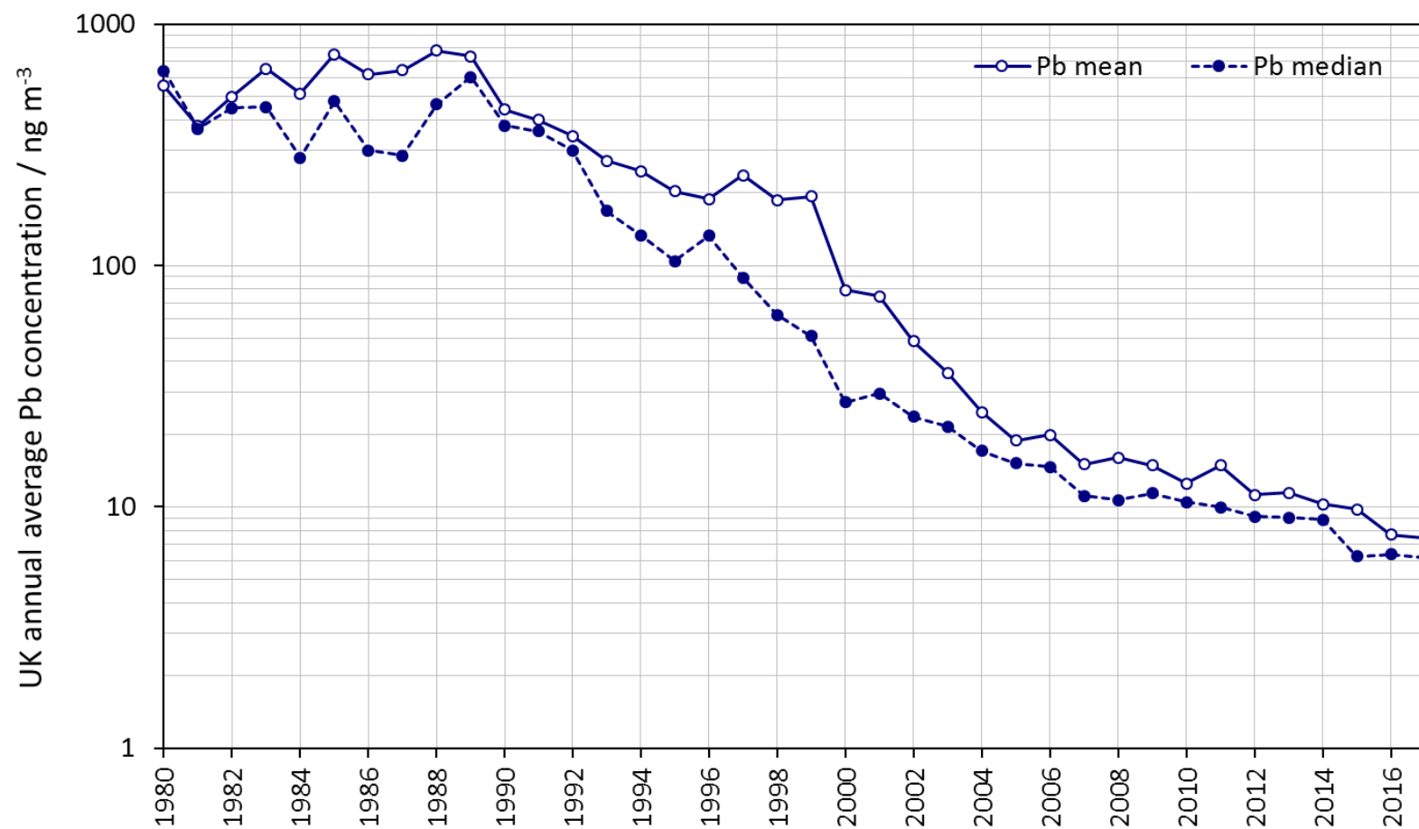
Figure 11. The mean and median of site annual average concentrations of Pb measured on the UK Heavy Metals Monitoring Network over the last 37 years. The EC limit value for lead is 500 \text{ ng m}^{-3} and the UK Air Quality Objective for lead is 250 \text{ ng m}^{-3} . Note the logarithmic scale on the y-axis.
