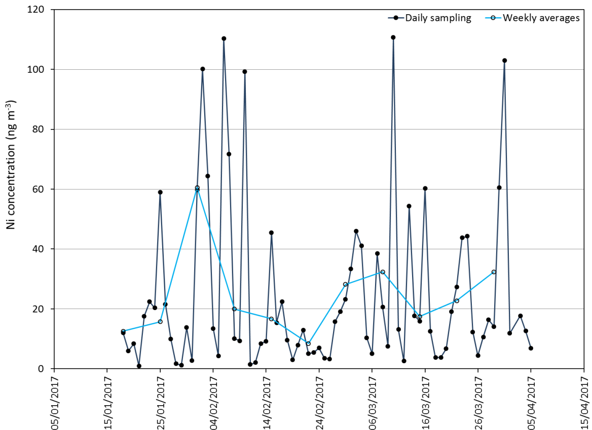
Figure 9. Comparing daily results and calculated weekly averages at Site 117: Sheffield Tinsley from 18 th January – 5 th April 2017.
