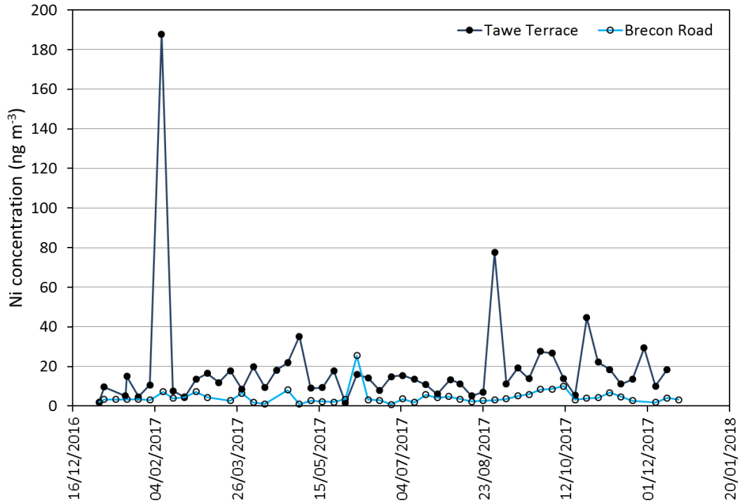
Figure 7. Measured Ni concentrations at Site 113: Pontardawe Tawe Terrace and Site 115: Pontardawe Brecon Road, in 2017 (both sampled weekly).
