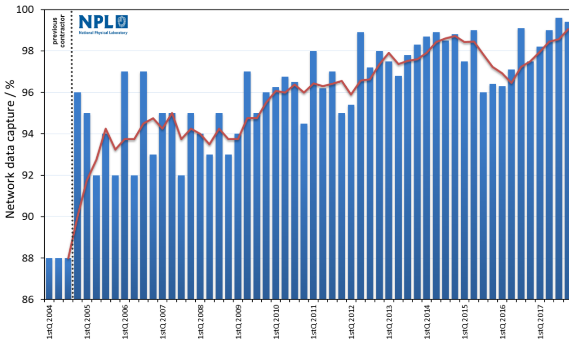
Figure 3. Network data capture from 2004-2017 (inclusive) for particulate and gaseous phase measurements. Quarterly data capture is indicated by the blue bars, whilst the rolling annual average data capture is given by the red line. Data to the right of the dotted vertical line is associated with NPL's current operation of the Network; data to the left of the dotted line is associated with the previous contractor's operation of the Network.
