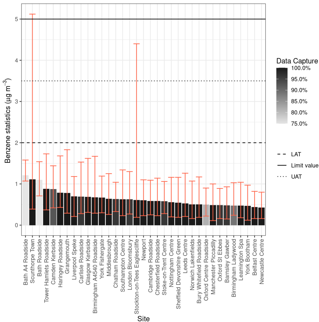
Figure 3: Non-Automatic Benzene annual statistics for 2019. Range shows the annual minimum and maximum.
