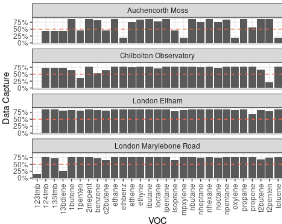
Figure 5: VOCs annual statistics for 2019. Dashed line shows the objective data capture rate.
