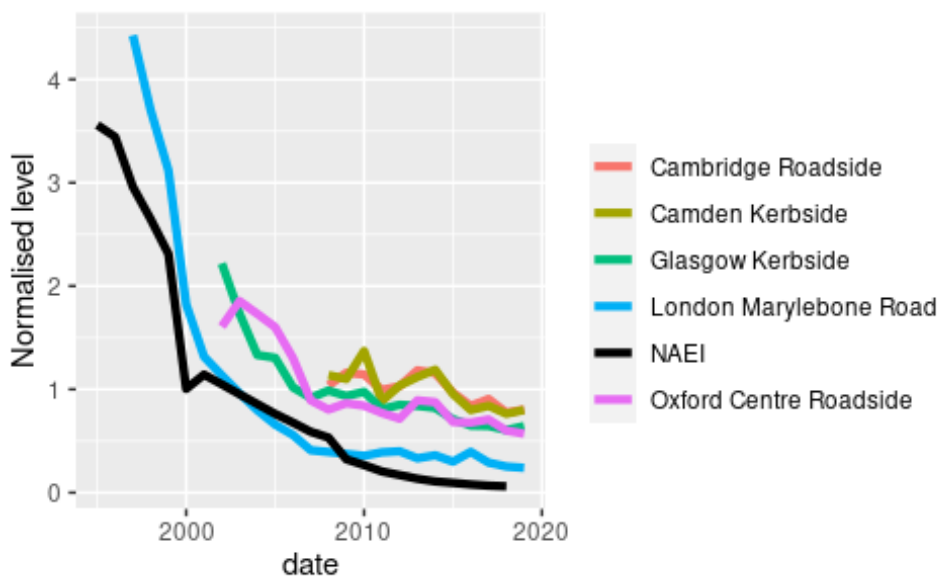
Figure 9: Normalised annual average benzene concentration and NAEI benzene emission estimate (1995 - 2019).
