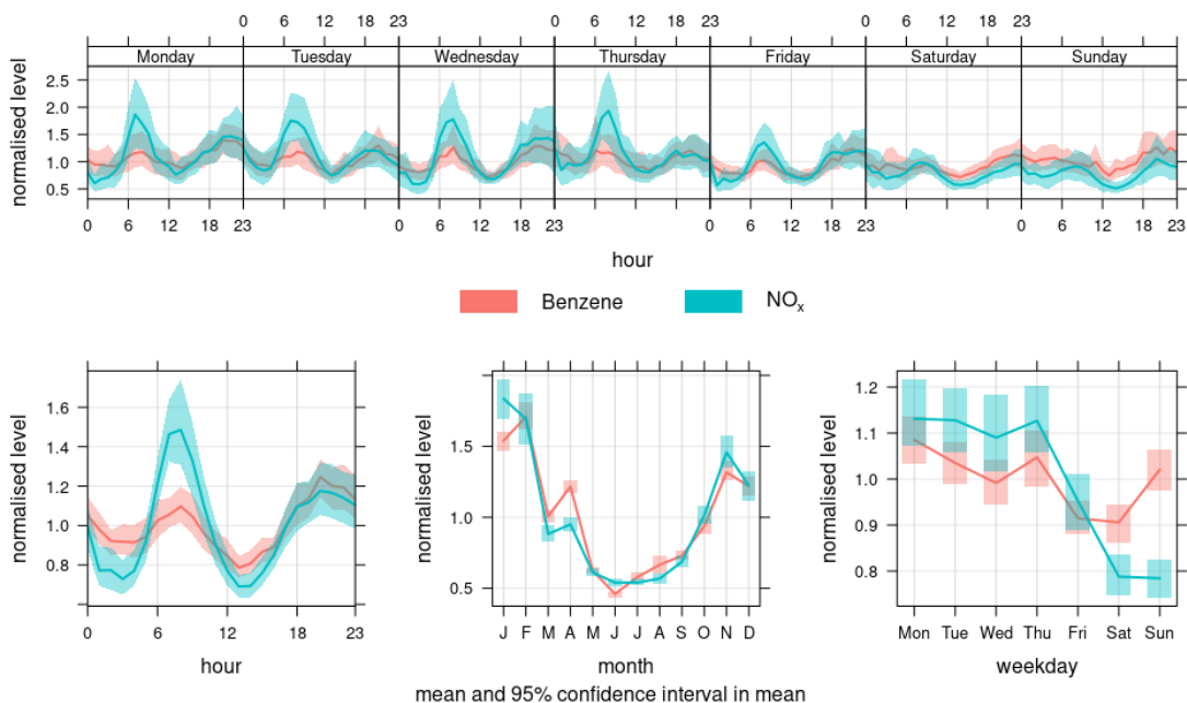
Figure 16: Diurnal, seasonal and week-daily variation of benzene and NO x at London Eltham.
