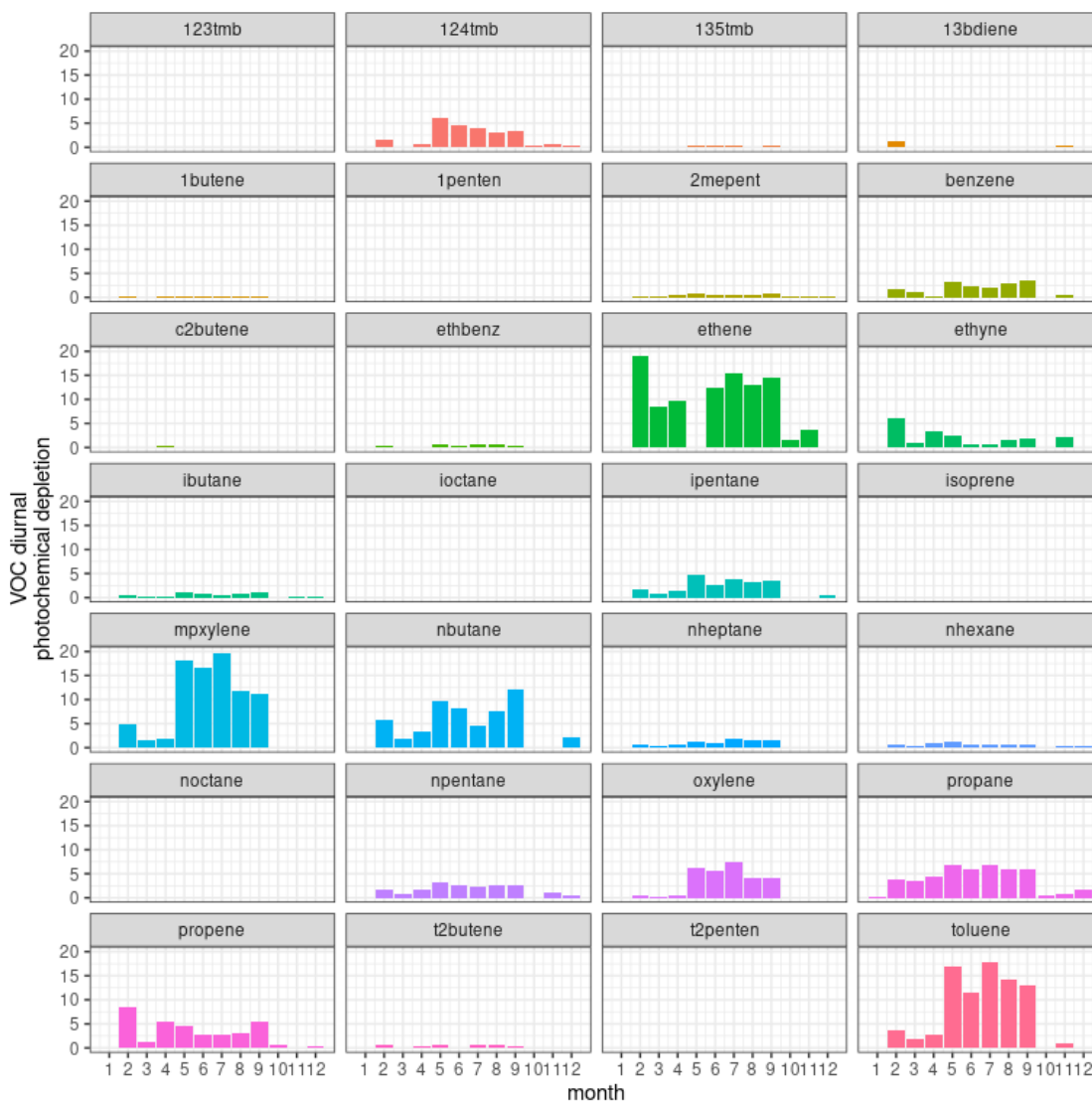
Figure 12: Median of the diurnal VOC photochemical depletion at Chilbolton for each month in 2019.
