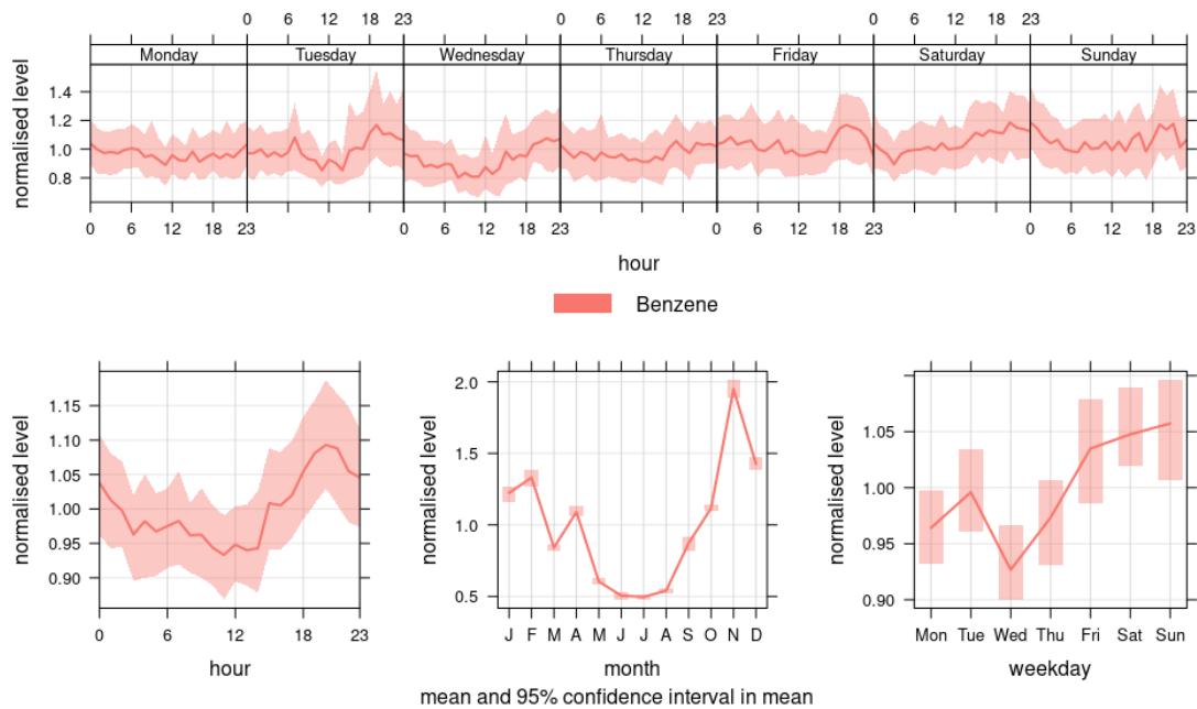
Figure 14: Diurnal, seasonal and week-daily variation of benzene at Auchencorth Moss.
