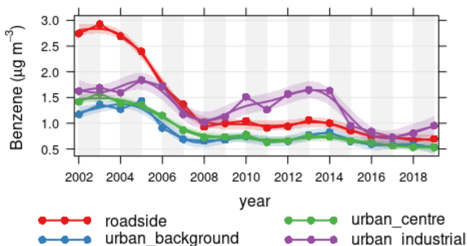
Figure 6: Average Non-Automatic network benzene means by site type from 2002 to 2019.
