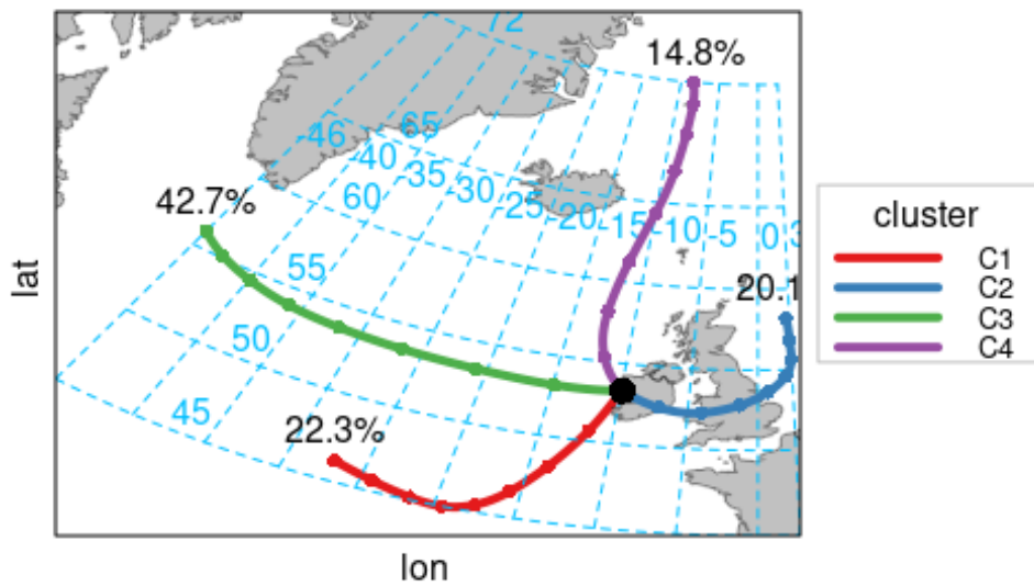
Figure 10: Air mass back trajectories arriving at Mace Head in 2019
