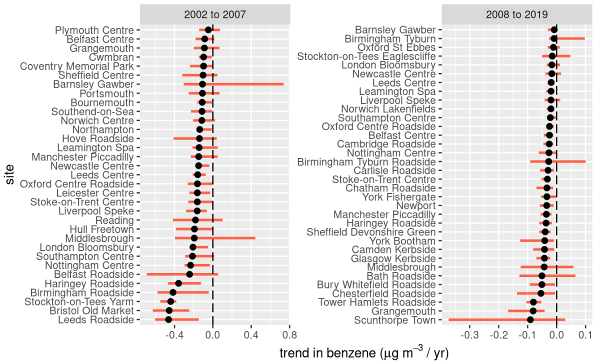
Figure 8: Benzene concentration trend ( \mu\text{g m}^{-3} / \text{yr} ) at non-automatic sites from 2002 to 2019.
