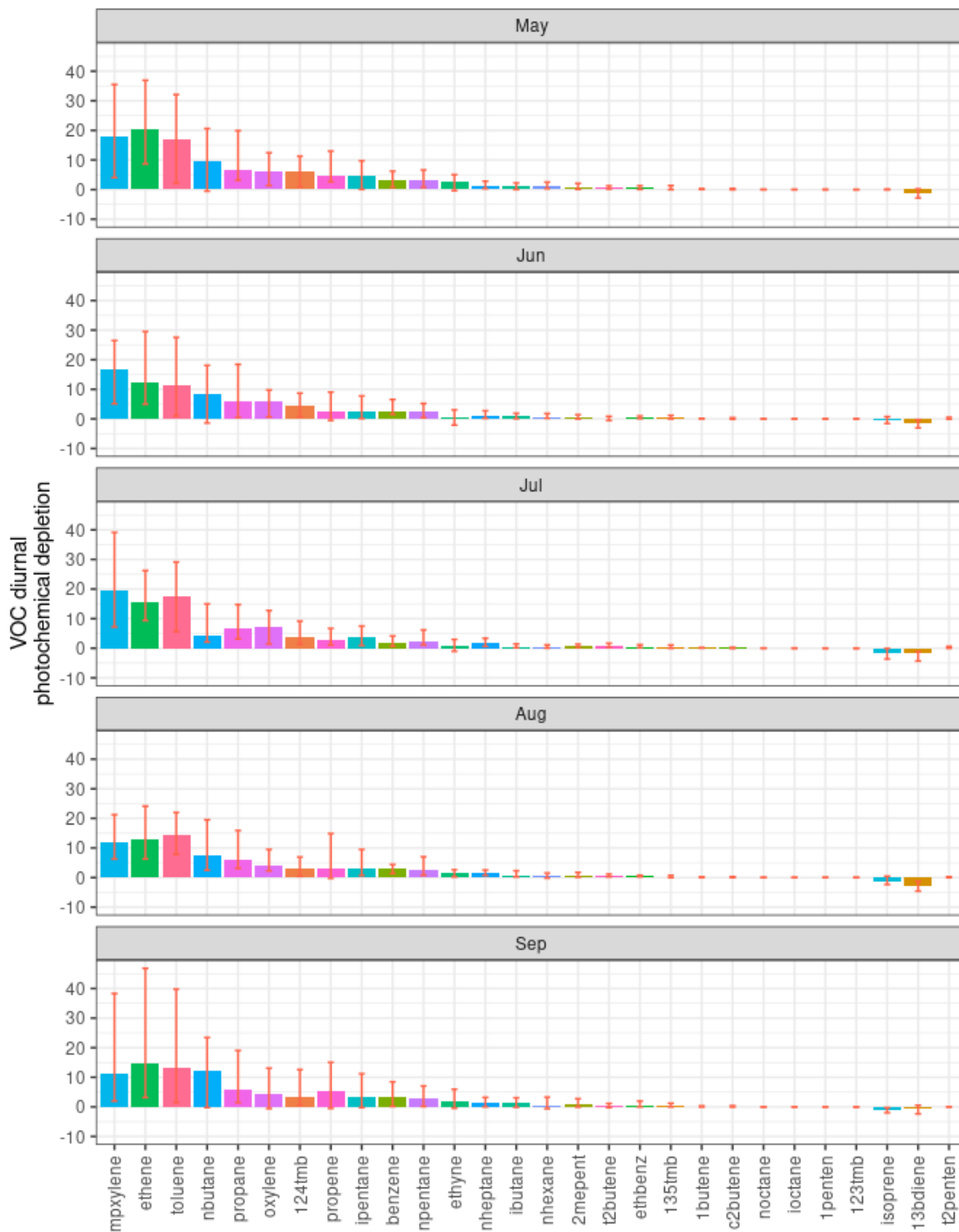
Figure 13: Median of the VOC diurnal photochemical depletion at Chilbolton between May and September in 2019. Error bar indicates the 25 and 75% percentile of the VOC diurnal photochemical depletion for a that VOC in the relevant month.
