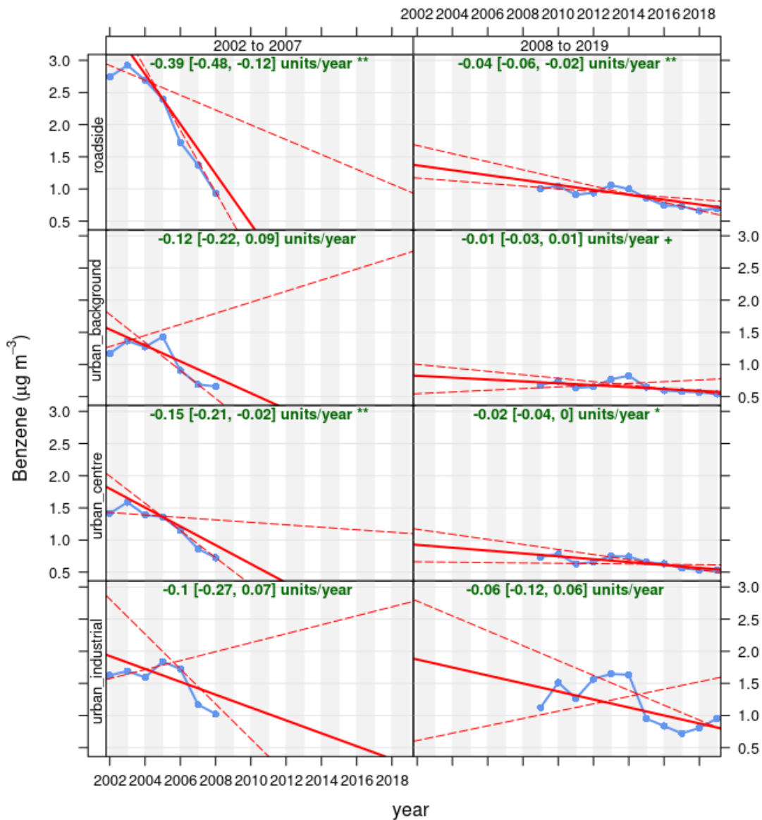
Figure 7: Non-automatic benzene rate of change for 2002-2007 and 2008-2019.
