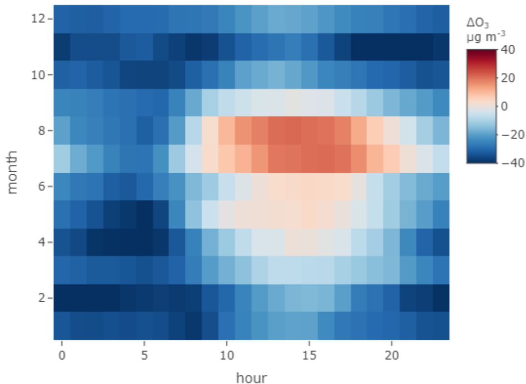
Figure 11: Month–hourly average differences between regional and hemispheric background O 3 for 2018 and 2019 at Chilbolton.
