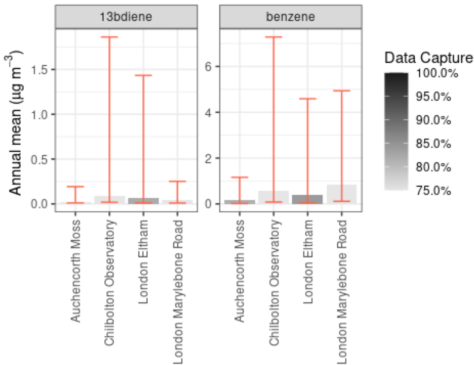
Figure 4: Benzene and 1,3-butadiene annual statistics for 2019. Range shows the annual minimum and maximum.
