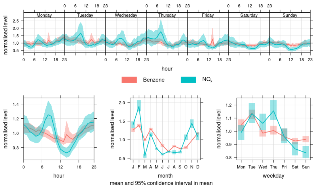
Figure 15: Diurnal, seasonal and week-daily variation of benzene, and NO x at Chilbolton.
