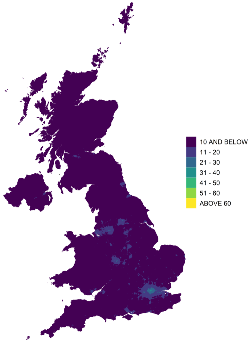
Figure 4.1 - Annual mean background NO 2 concentration, 2021 ( \mu\text{g m}^{-3} )
