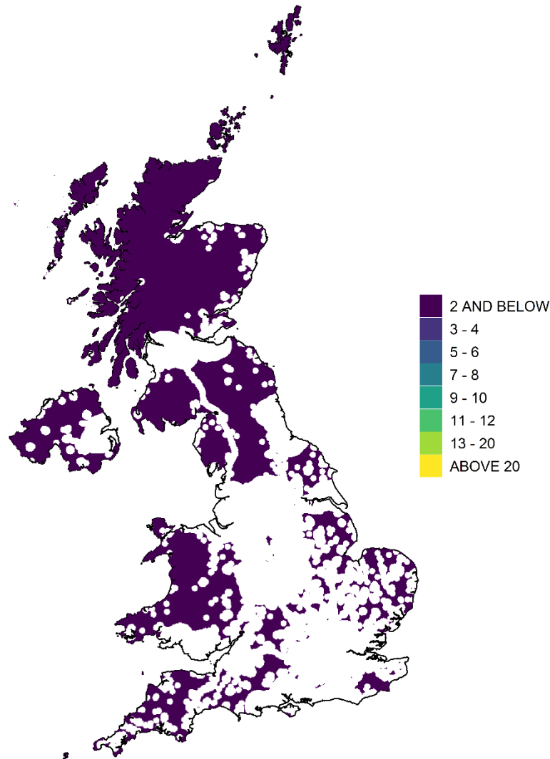
Figure 5.2 - Annual mean SO 2 concentration, 2021 (µg m -3 ) in vegetation areas
