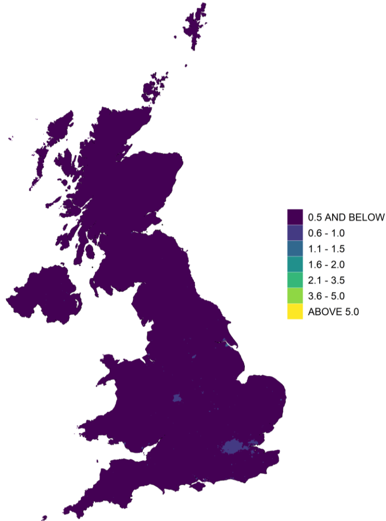
Figure 8.2 - Annual mean background benzene concentration, 2021 ( \mu\text{g m}^{-3} )
