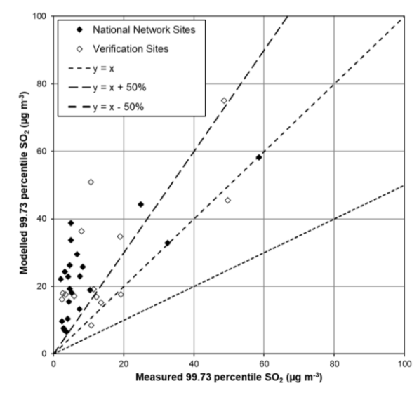
Figure 5.13 - Verification of 99.73 percentile of 1-hour mean SO 2 model, 2021
