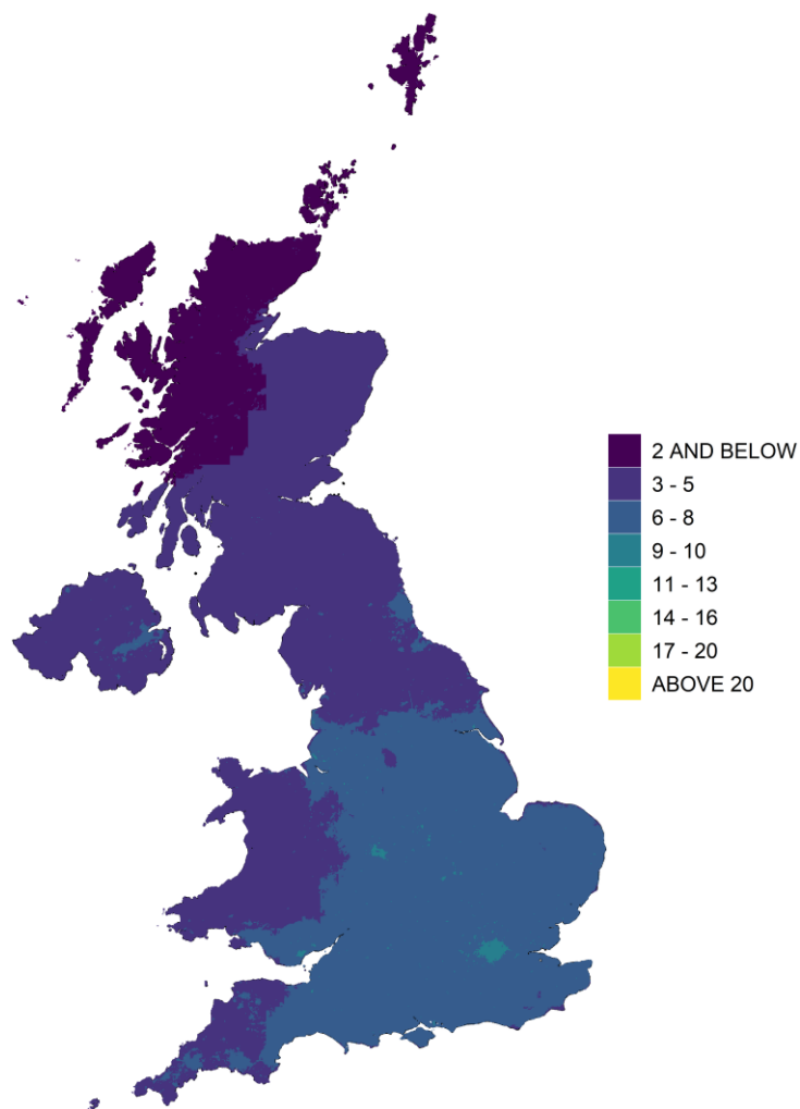
Figure 7.1 - Annual mean background PM 2.5 concentration, 2021 ( \mu\text{g m}^{-3} , gravimetric)
