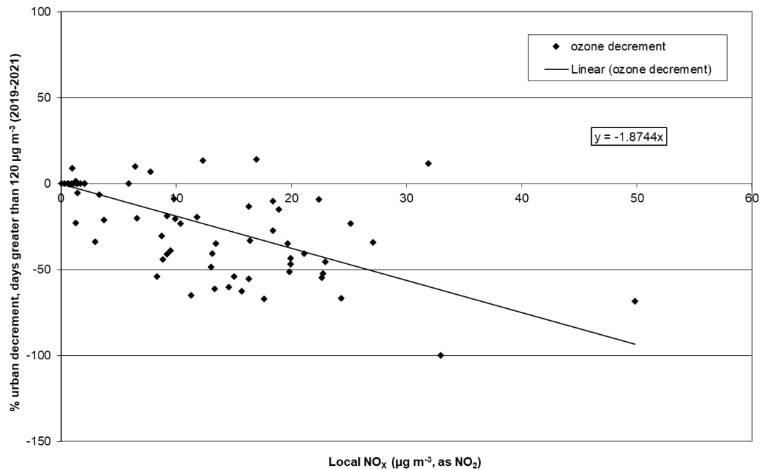
Figure 10.5 - Days greater than 120 \mu\text{g m}^{-3} percentage decrement in ozone concentrations, 2019-2021
