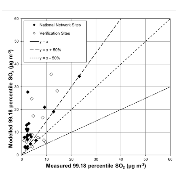
Figure 5.14 - Verification of 99.18 percentile of 24-hour mean SO 2 model, 2021
