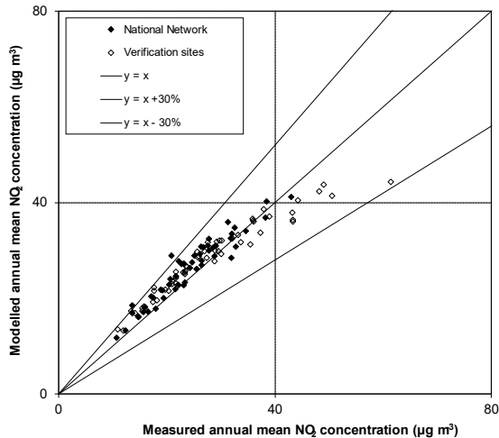
Figure 4.15 - Verification of roadside relationship at roadside locations in 2021
