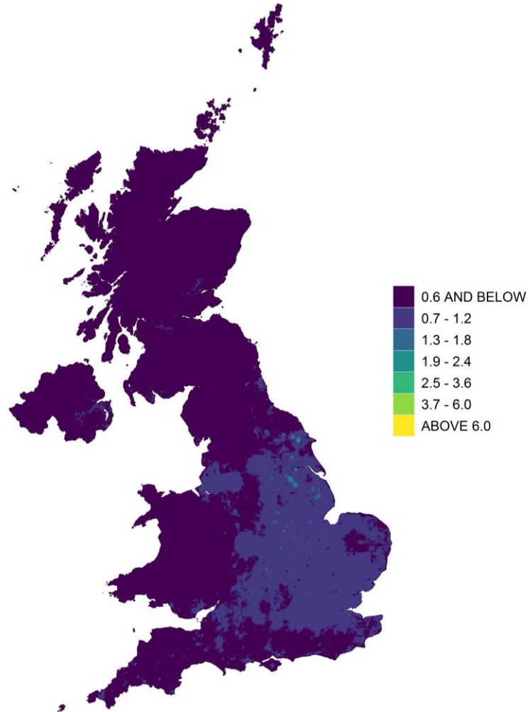
Figure 11.2 - Annual mean background As concentration, 2021 (ng m -3 )
