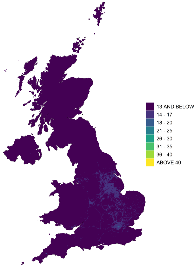
Figure 6.1 - Annual mean background PM 10 concentration, 2021 ( \mu\text{g m}^{-3} , gravimetric)
