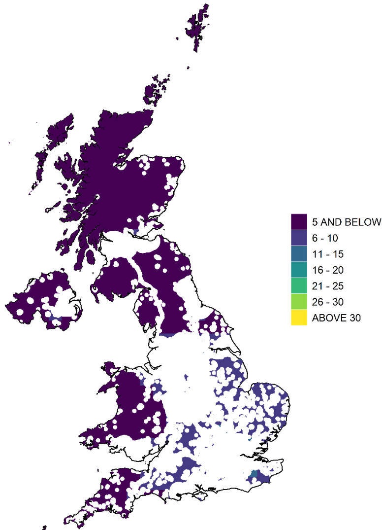
Figure 4.3 - Annual mean map of NO x concentrations for comparison with the NO x vegetation critical level, 2021 (µg m -3 , as NO 2 )
