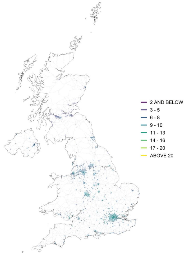
Figure 7.2 - Urban major roads, annual mean roadside PM 2.5 concentration, 2021 ( \mu\text{g m}^{-3} , gravimetric)
