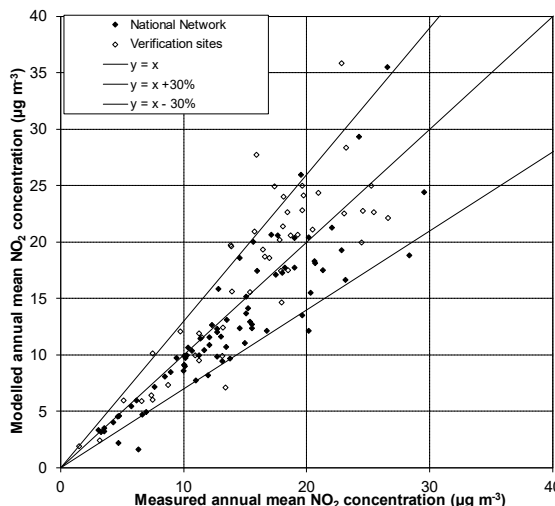
Figure 4.19 - Verification of roadside annual mean NO 2 model 2021
