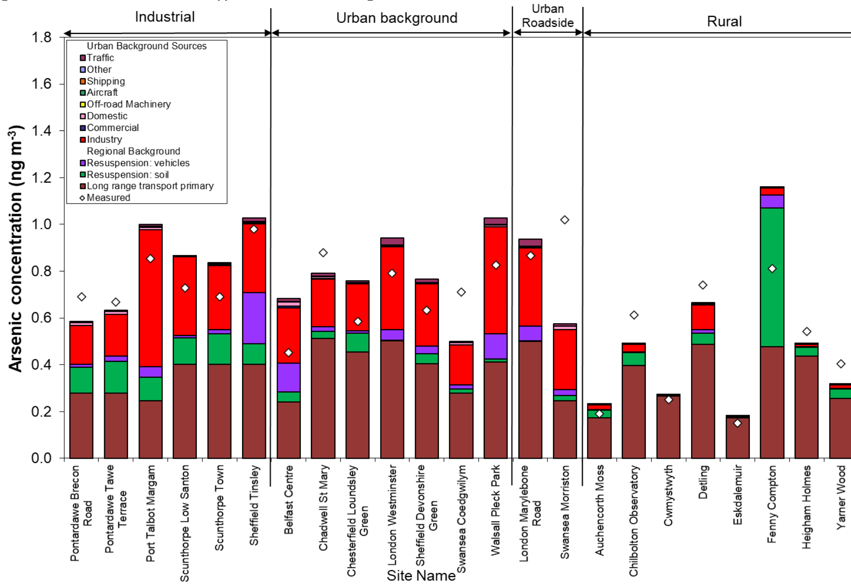
Figure 11.11 - Annual mean As source apportionment at monitoring sites in 2021.
