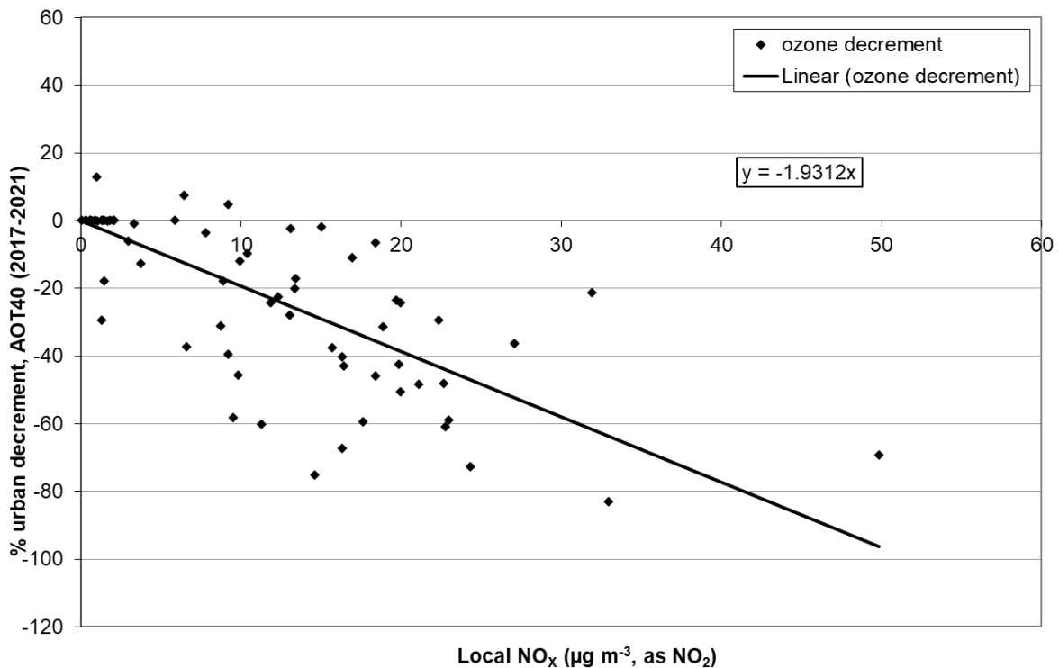
Figure 10.11 - AOT40 percentage decrement in ozone concentrations, 2017-2021
