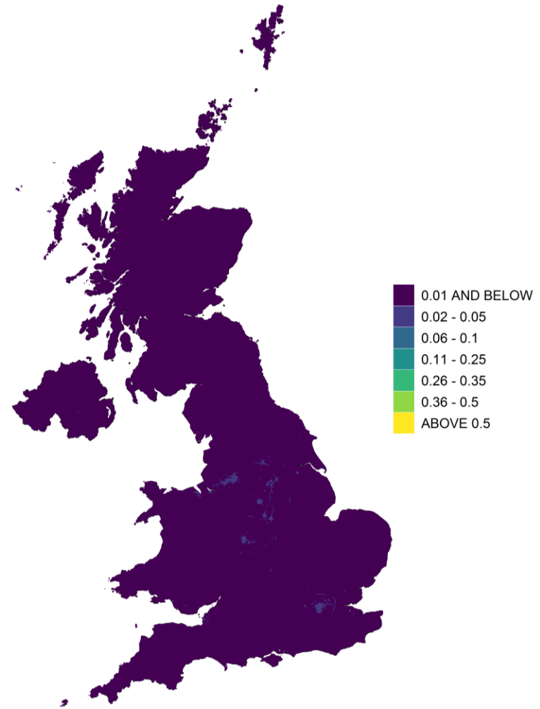
Figure 11.5 - Annual mean background Pb concentration, 2021 ( \mu\text{g m}^{-3} )
