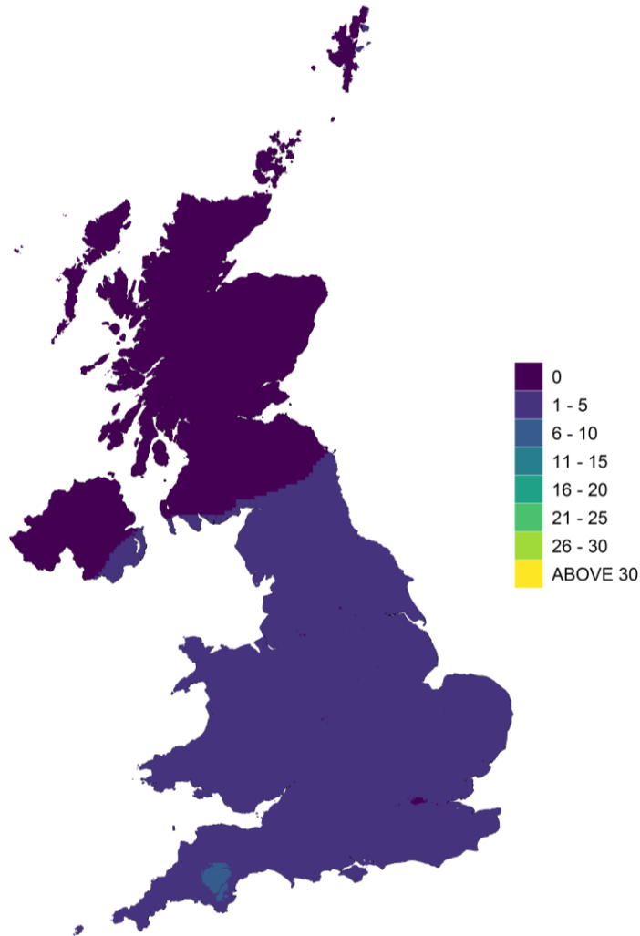
Figure 10.2 - Estimated number of days with an 8-hour mean ozone concentration above 120 \mu\text{g m}^{-3} , 2021
