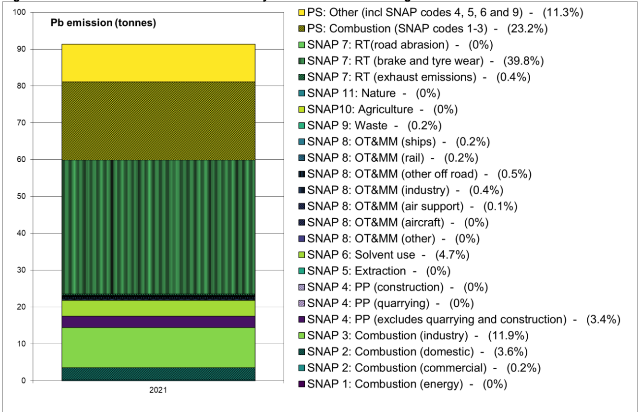
Figure 11.9 - Total UK Pb emissions for 2021 by SNAP code scaled using Covid factors from NAEI 2020
