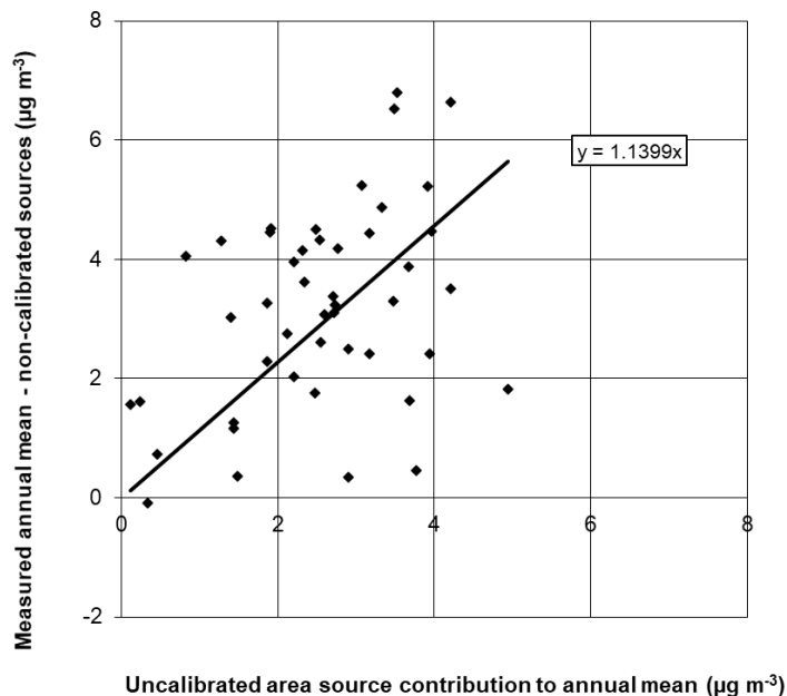
Figure 6.8 - Calibration of PM 10 area source model 2021 (µg m -3 , gravimetric)
