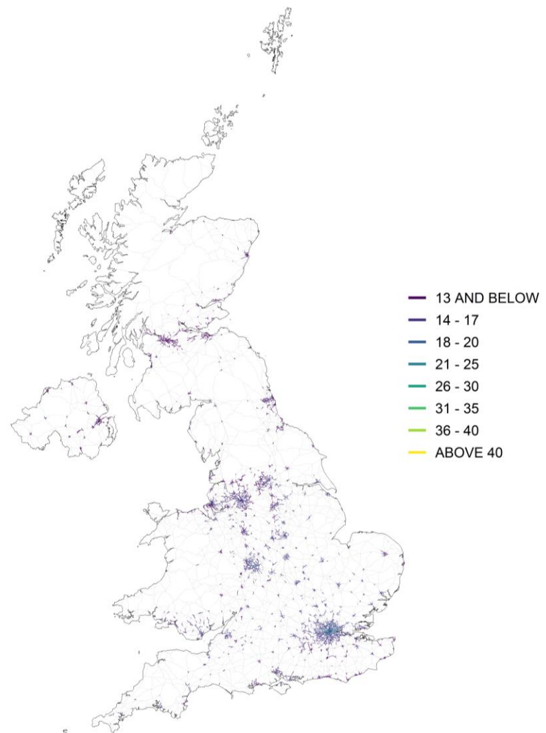
Figure 6.2 - Urban major roads, annual mean roadside PM 10 concentration, 2021 ( \mu\text{g m}^{-3} , gravimetric)
