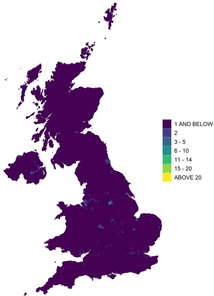
Figure 11.4 - Annual mean background Ni concentration, 2021 ( \text{ng m}^{-3} )
