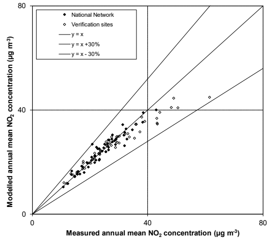
Figure 4.15 - Verification of roadside relationship at roadside locations in 2021
