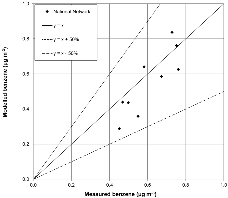
Figure 8.8 - Verification of roadside annual mean benzene model 2021
