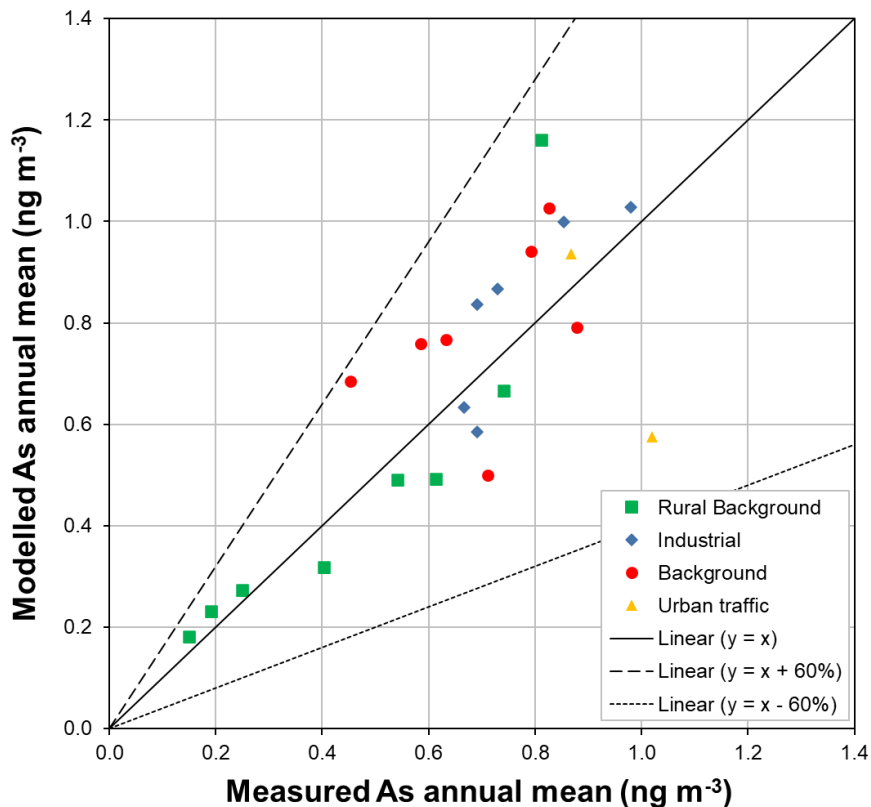
Figure 11.10 - Verification of annual mean As across all sites.
