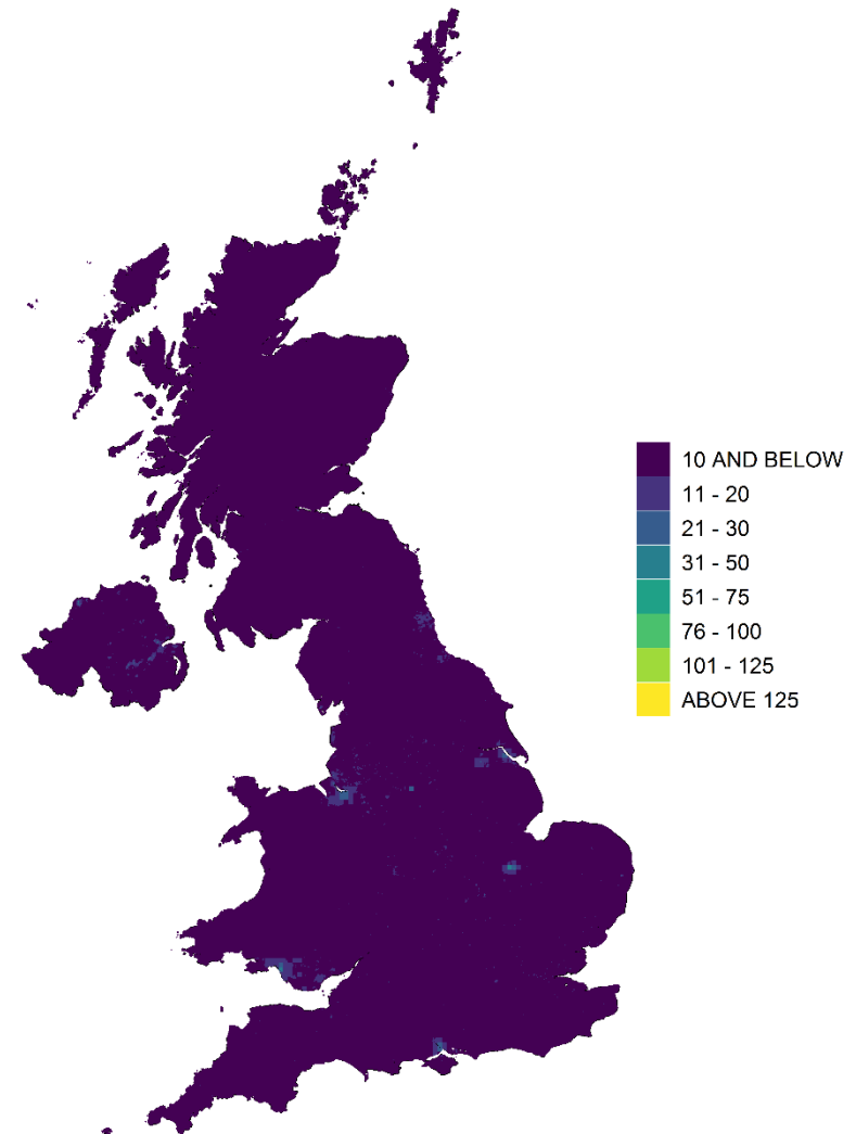
Figure 5.5 - 99.18 percentile of 24-hour mean SO 2 concentration, 2021 ( \mu\text{g m}^{-3} )
