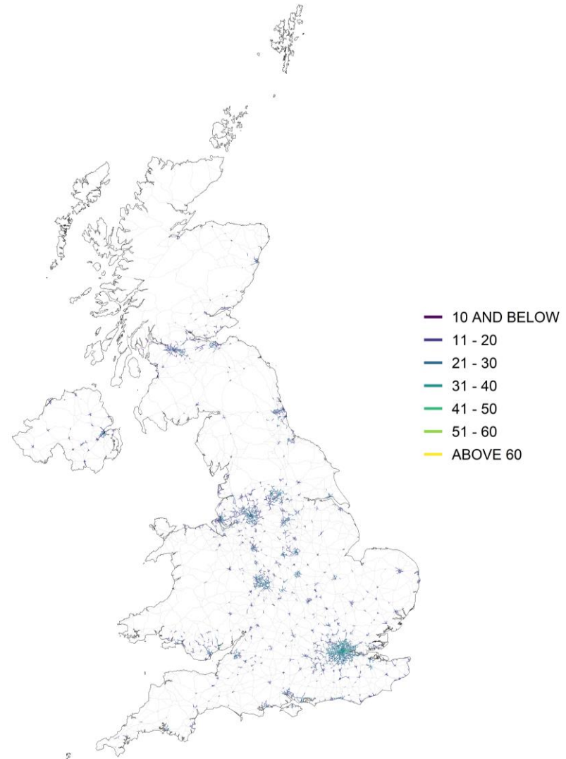
Figure 4.2 - Urban major roads, annual mean roadside NO 2 concentration, 2021 ( \mu\text{g m}^{-3} )
