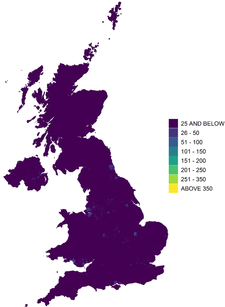
Figure 5.4 - 99.73 percentile of 1-hour mean SO 2 concentration, 2021 ( \mu\text{g m}^{-3} )
