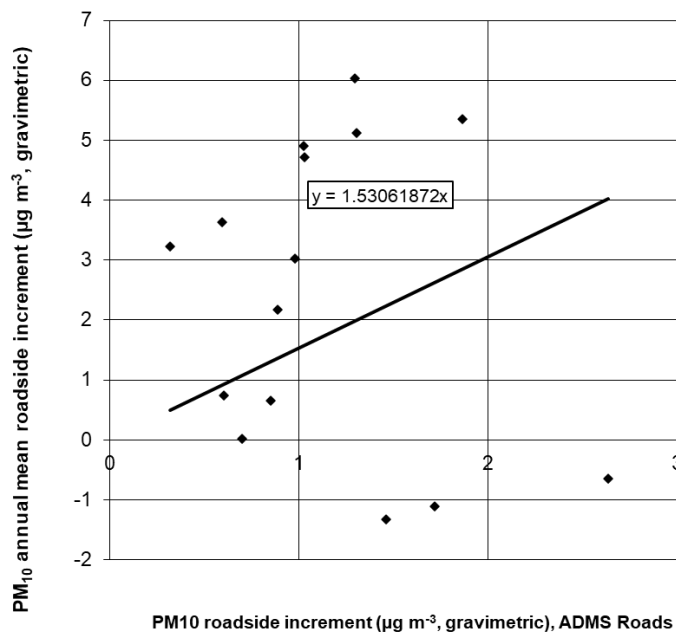
Figure 6.9 - Calibration of PM 10 PCM-RKM model 2021 (µg m -3 , gravimetric)
