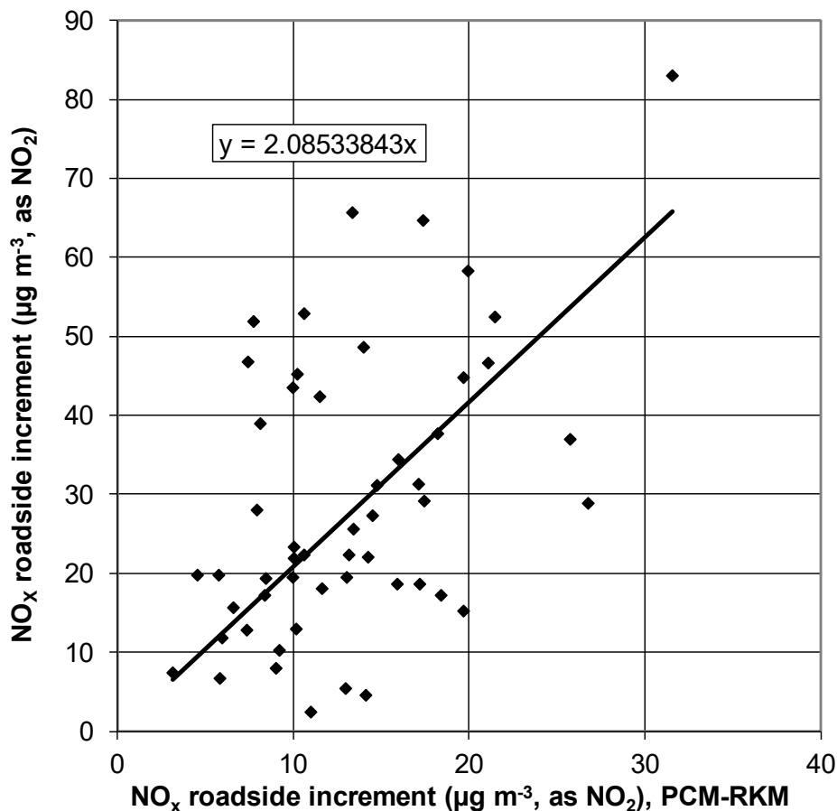
Figure 4.9 - Calibration of NO x PCM RKM model, 2021 (µg m -3 , as NO 2 )
