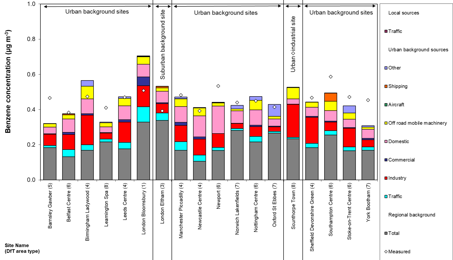
Figure 8.9 - Annual mean benzene source apportionment at background monitoring sites in 2021 (the area type of each site is shown in parenthesis after its name)
