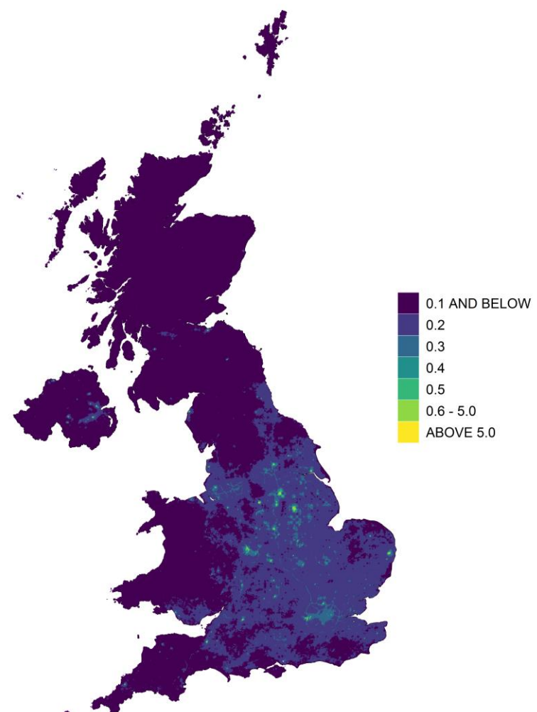
Figure 11.3 - Annual mean background Cadmium (Cd) concentration, 2021 (ng m -3 )
