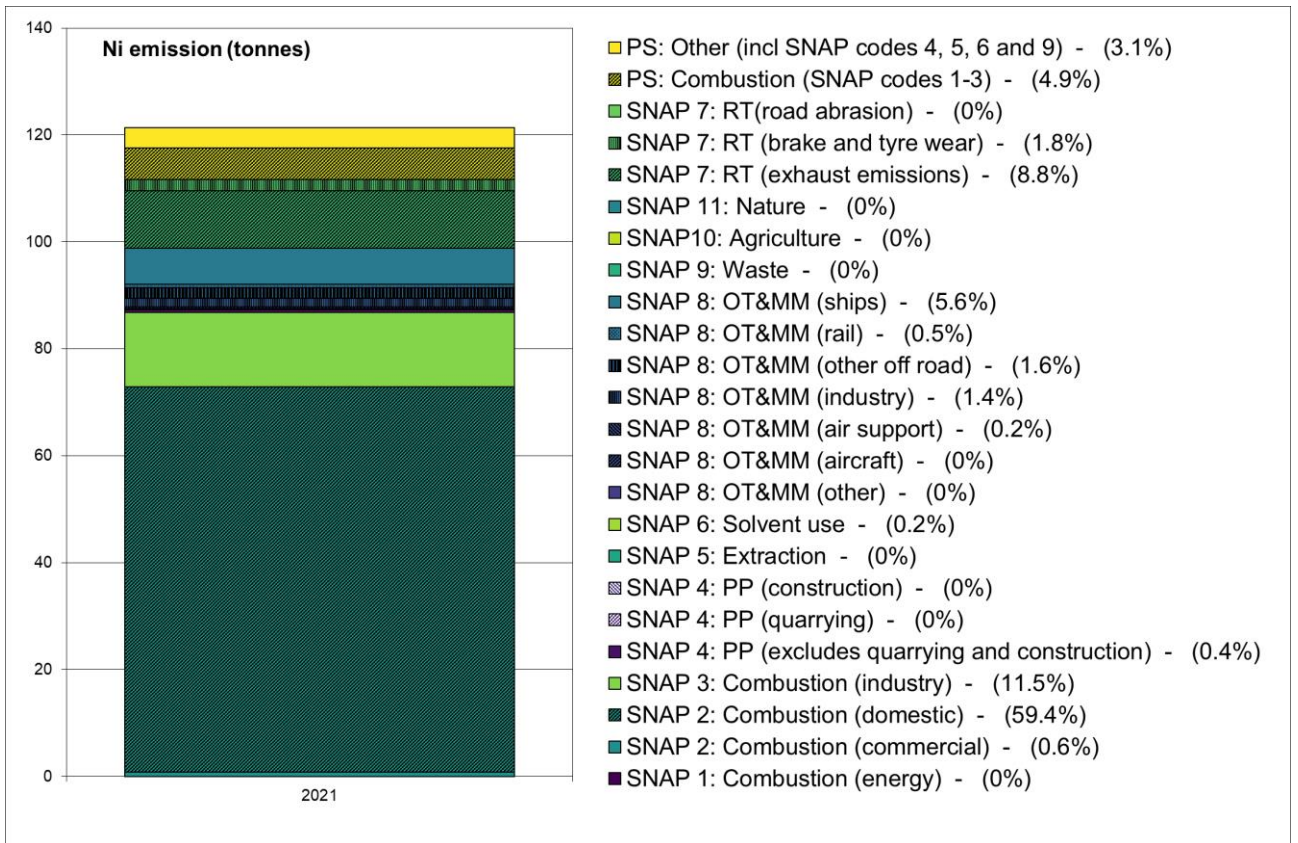
Figure 11.8 - Total UK Ni emissions for 2021 by SNAP code scaled using Covid factors from NAEI 2020
