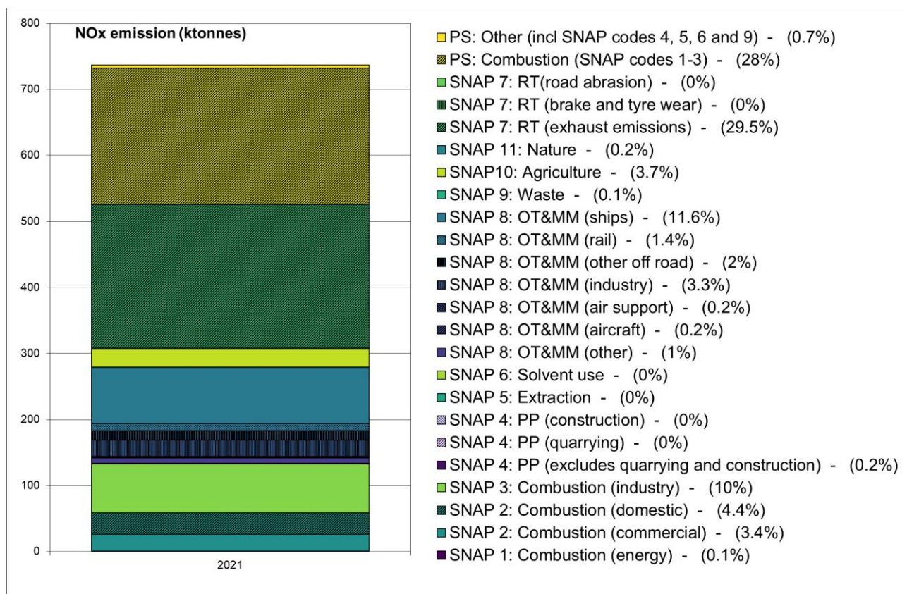
Figure 4.6 - Total UK NO x emissions for 2021 by SNAP code scaled using Covid factors from NAEI 2020
