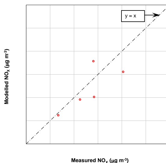
Figure A6.2 - Comparison of the measured and modelled annual mean NO x at Gatwick Airport for 2008
