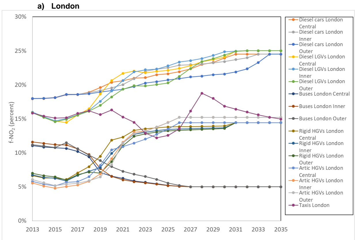
Figure 4.10 - Fleet average f-NO 2 projections by vehicle type for a) London and b) rest of the UK from NAEI
