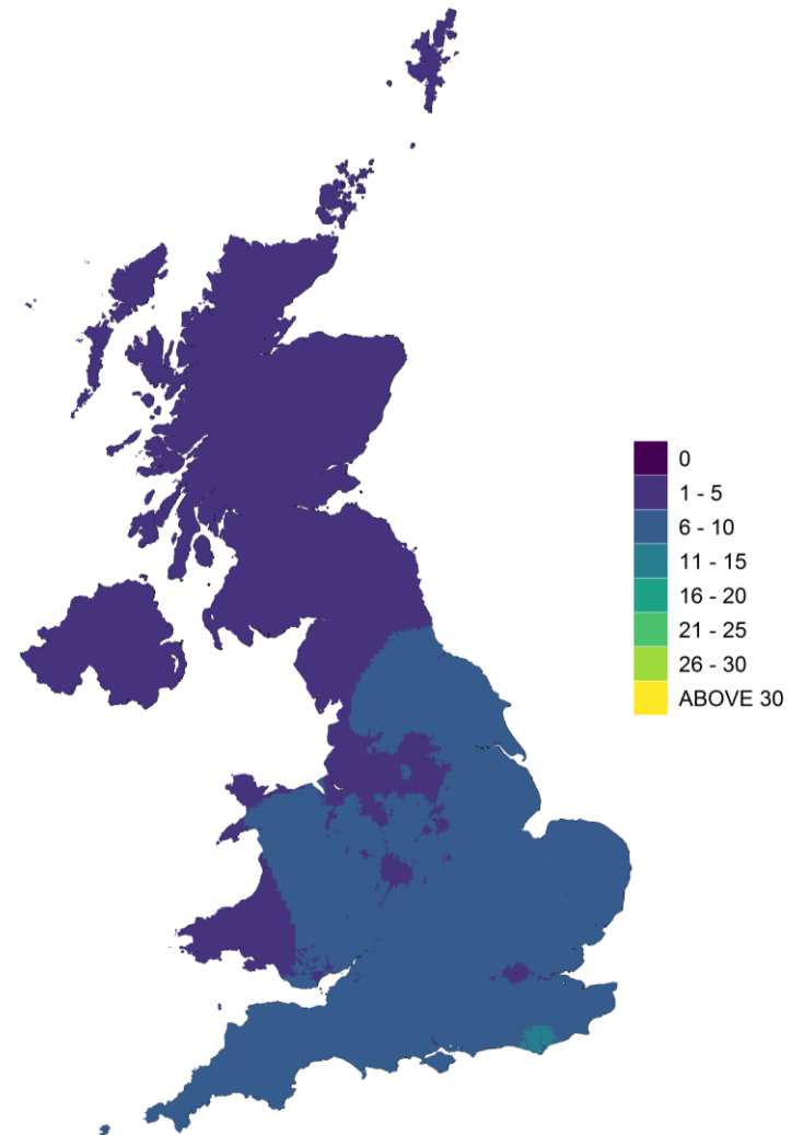
Figure 10.3 - Estimated average number of days with an 8-hour mean ozone concentration above 120 \mu\text{g m}^{-3} , 2019 to 2021
