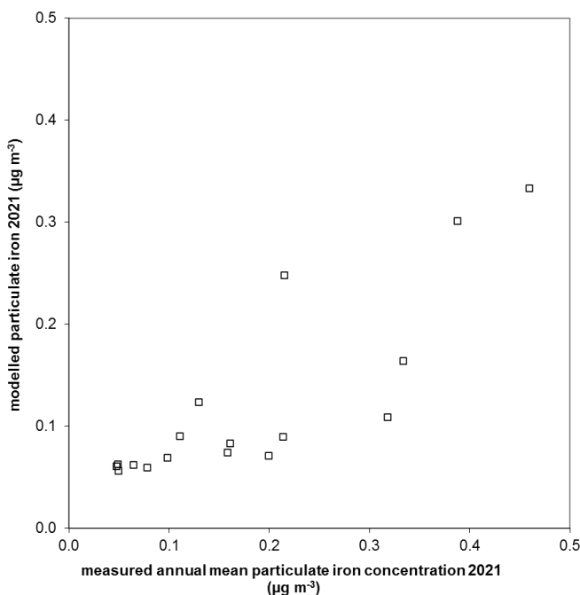
Figure 6.7 - Comparison of modelled and measured annual mean elemental Fe concentrations 2021 ( \mu\text{g m}^{-3} )
