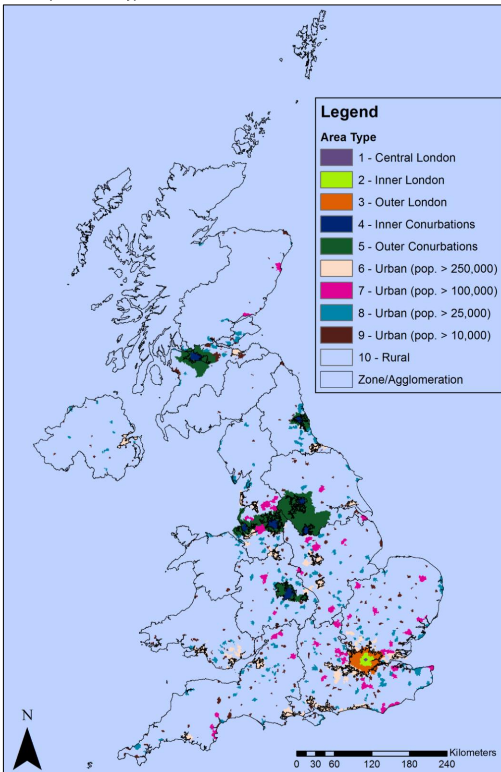
Figure A5.4 - Map of UK area types
