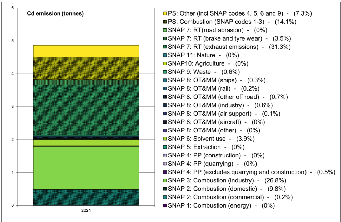
Figure 11.7 - Total UK Cd emissions for 2021 by SNAP code scaled using Covid factors from NAEI 2020
