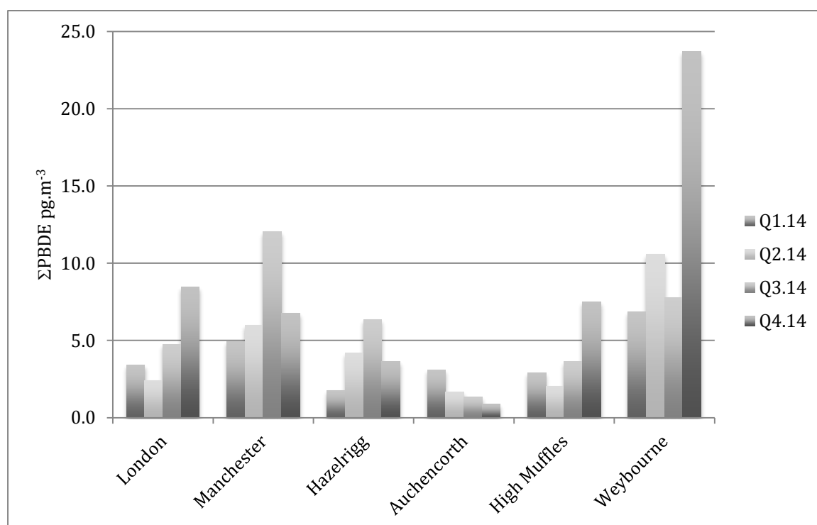
Figure 7. Quarterly \Sigma PBDE data at the TOMPs sites for 2014.
