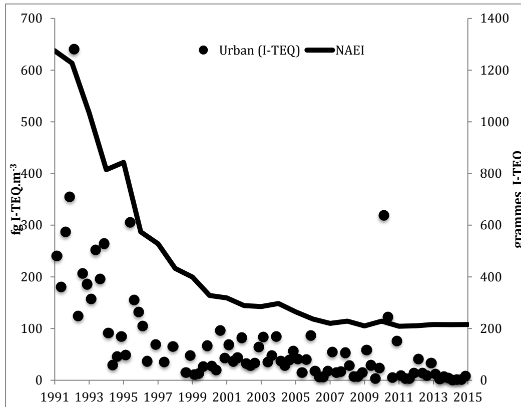
Figure 3. Long-term PCDD/F trend data in fg I-TEQ.m -3 from the TOMPs network for the urban (London and Manchester) and the rural (Hazelrigg, High Muffles, Auchencorth and Weybourne) sites. Quarterly data are compared to the current NAEI estimates in g I-TEQ per annum.
