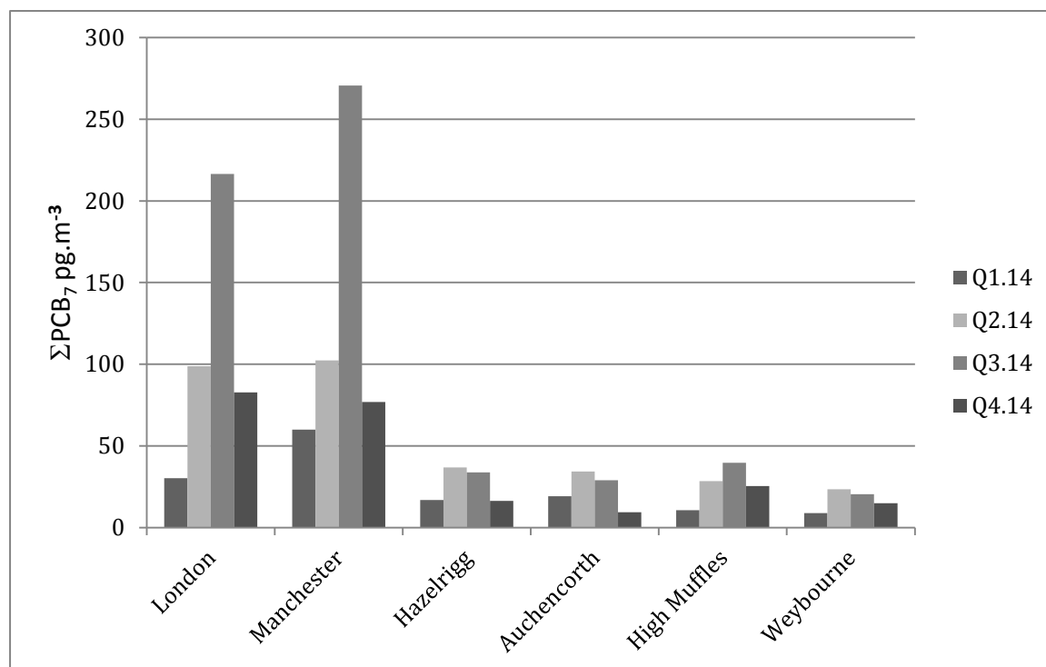
Figure 5. Quarterly \Sigma\text{PCB}_7 (congeners 28, 52, 101, 118, 153, 138 and 180) data at the TOMPs sites for 2014.
