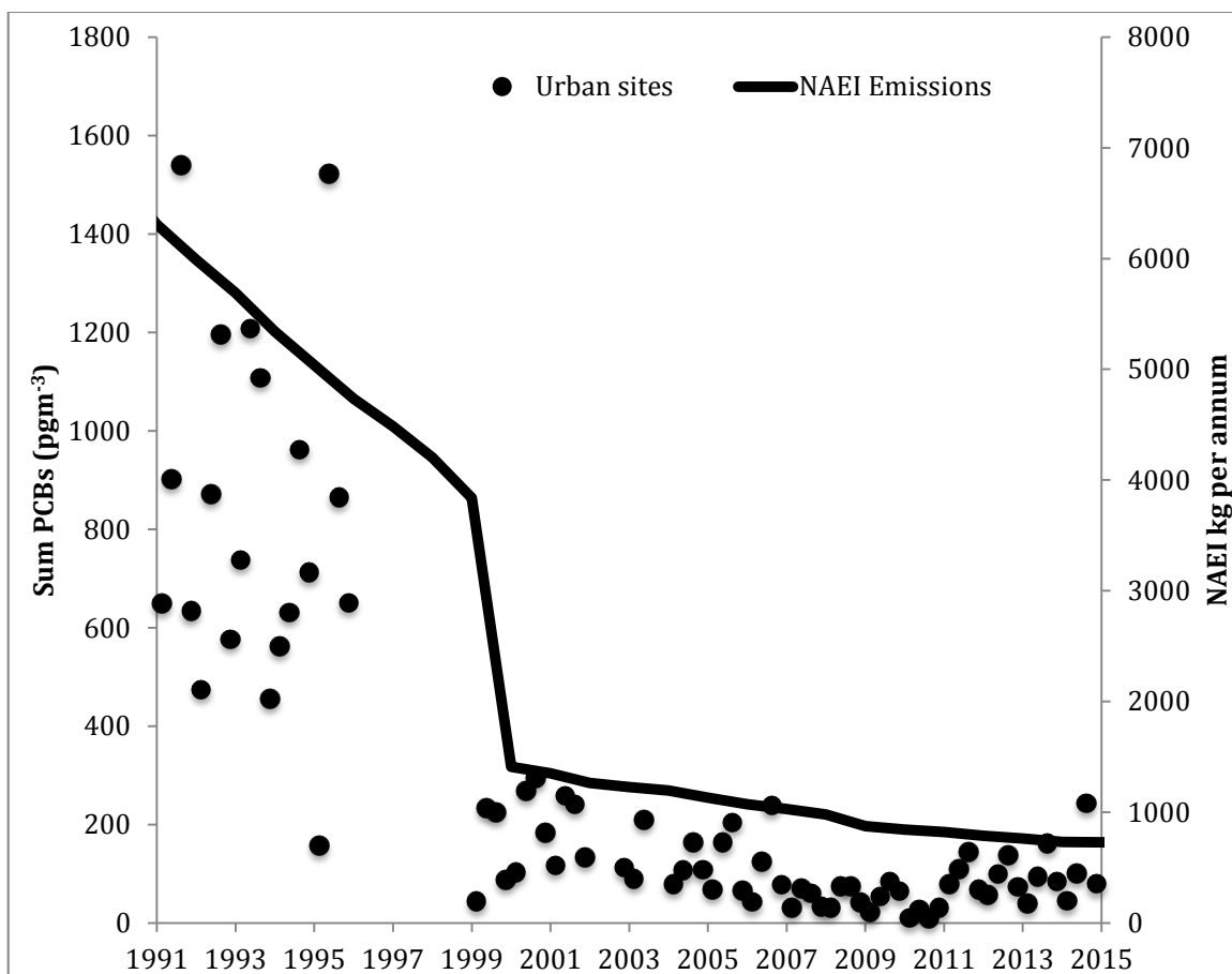
Figure 6. \Sigma_7 PCB Long-term PCB trend data from the TOMPs network for the urban (London and Manchester) and the rural (Hazelrigg, High Muffles, Auchencorth and Weybourne) sites. Data are presented as averages in \text{pgm}^{-3} and compared to the current NAEI estimates in kg per annum
