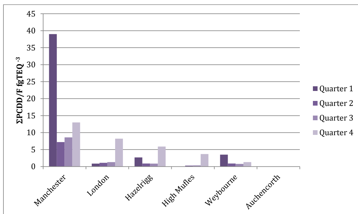
Figure 2. Quarterly PCDD/F data for each TOMPs site in 2014.
